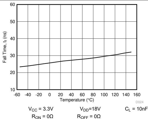
FIG 6-17. t_f Fall Time vs Temperature
