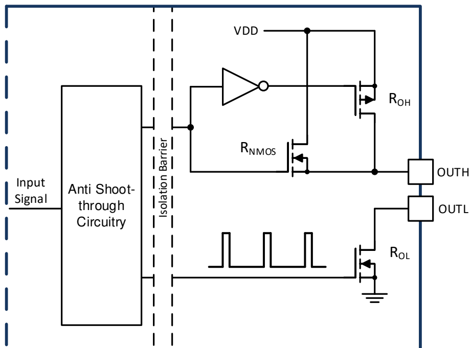
8-1. Gate Driver Output Stage
