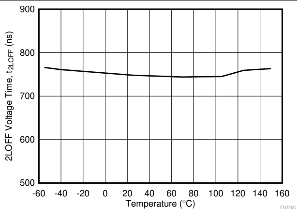
FIG 5-28. t 2LOFF 2-Level Turn Off Time vs Temperature
