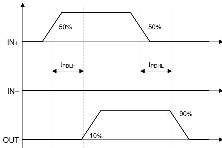
FIG 6-1. Non-inverting Logic Propagation Delay Measurement
