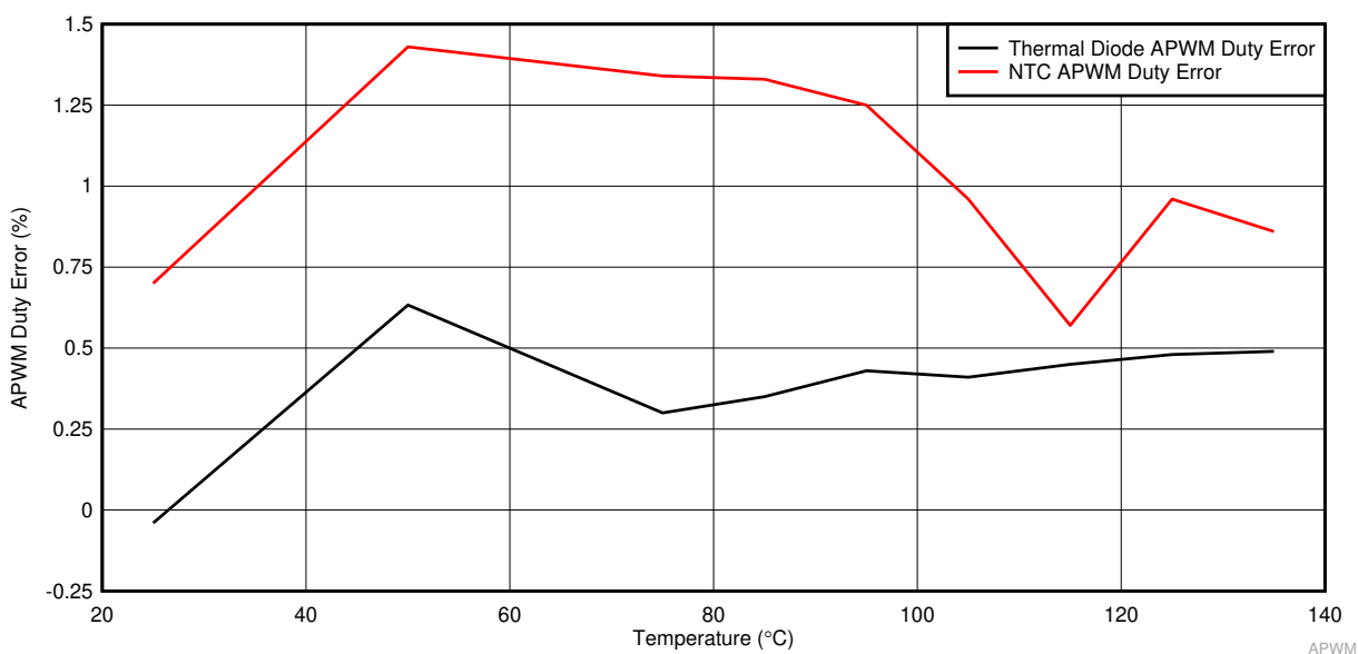
Figure 8-14. APWM Duty Error Without Calibration
