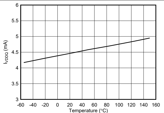
図 6-9. I_{VDDQ} Supply Current vs Temperature
