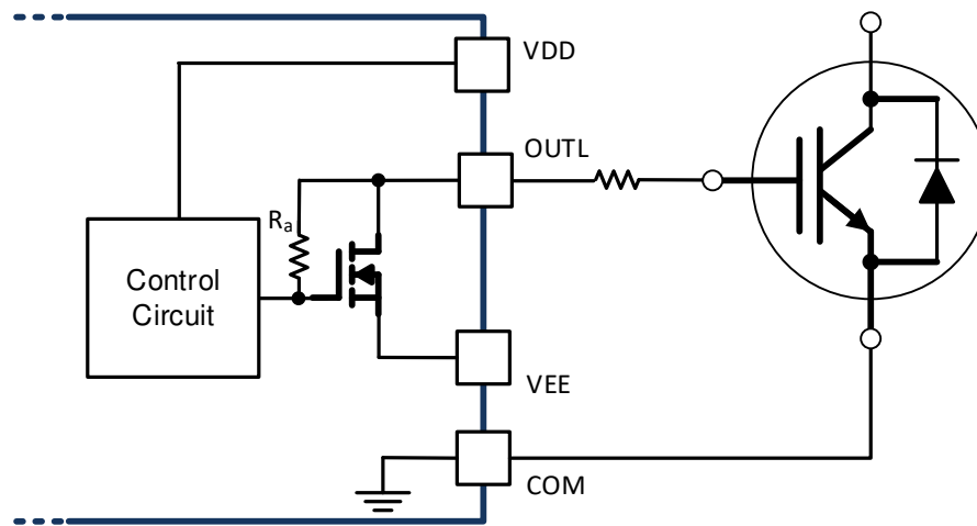
8-2. Active Pulldown
