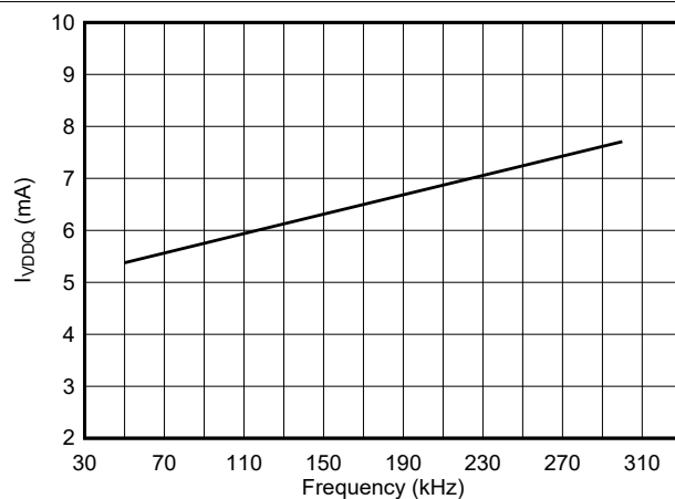
図 6-11. I_{VDDQ} Supply Current vs Input Frequency
