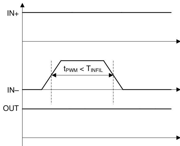
図 7-5. IN− ON Deglitch Filter
