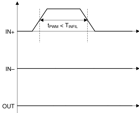
図 7-3. IN+ ON Deglitch Filter
