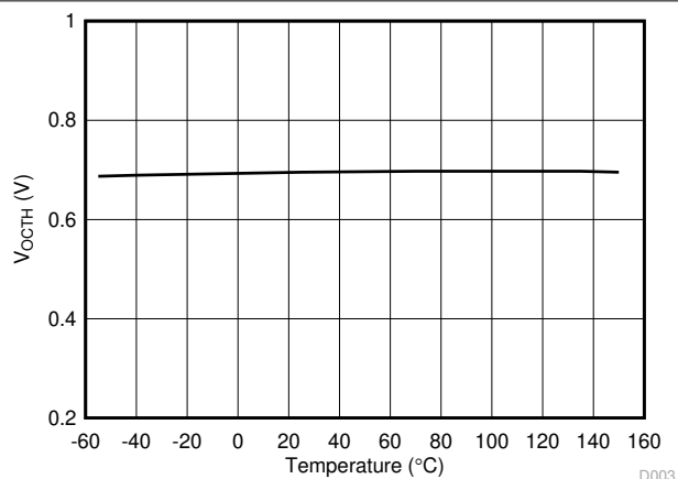
図 6-24. V_{OCTH} OC Detection Threshold vs Temperature
