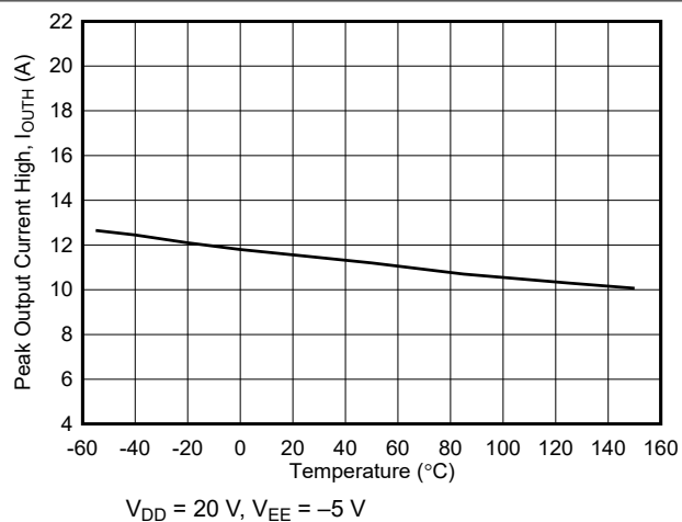
図 6-4. Output High Drive Current vs Temperature
