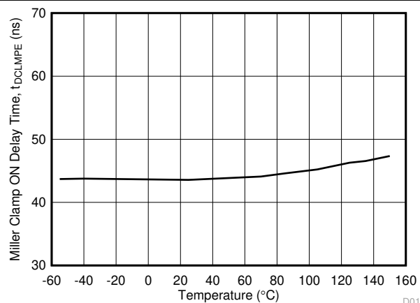
图 6-23. t_{DCLMPE} Miller Clamp ON Delay Time vs Temperature
