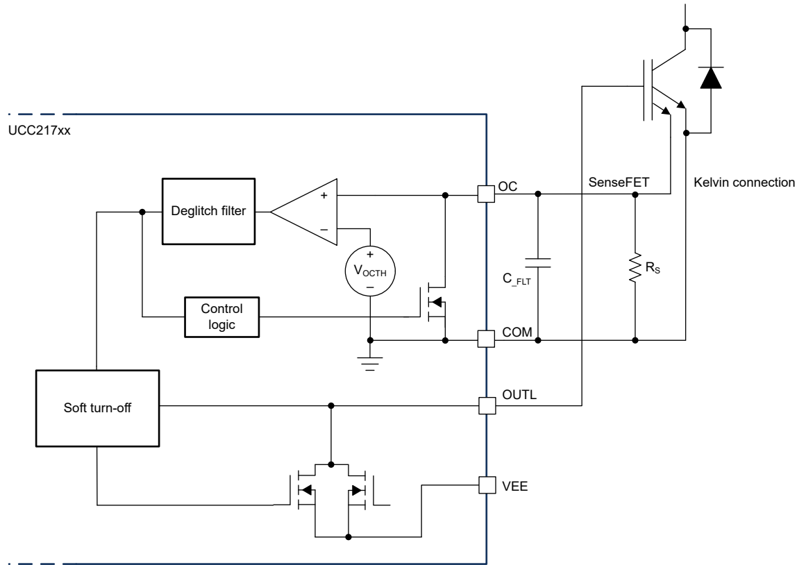
☒ 8-6. Soft Turn-off
