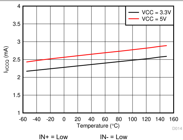
図 6-7. I_{VCCQ} Supply Current vs Temperature
