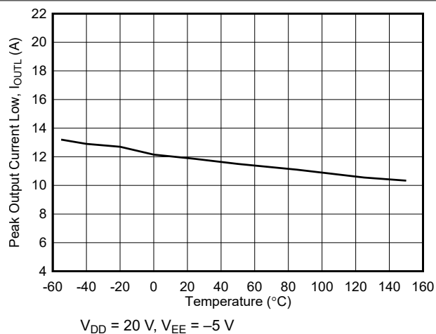
図 6-5. Output Low Driver Current vs Temperature
