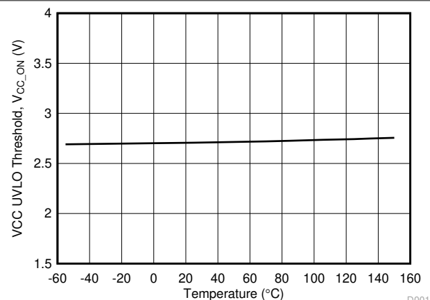
図 6-12. VCC UVLO vs Temperature
