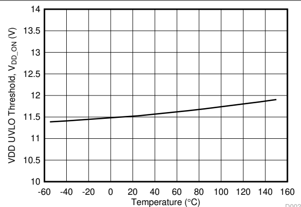
図 6-13. VDD UVLO vs Temperature
