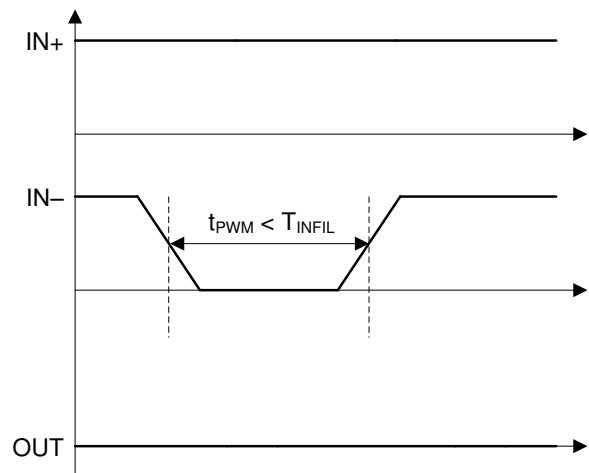
図 7-6. IN− OFF Deglitch Filter
