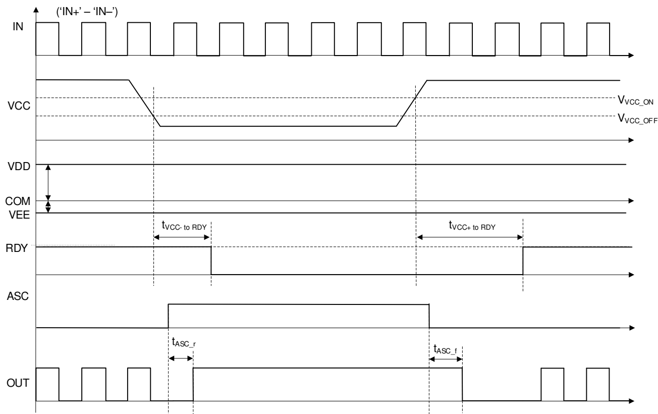
図 7-11. ASC Support with VCC UVLO
