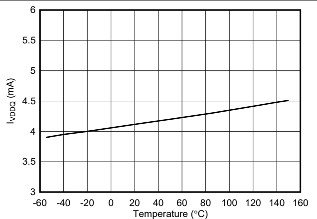
図 6-10. I_{VDDQ} Supply Current vs Temperature
