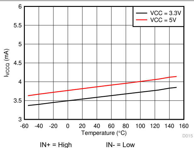
図 6-6. I_{VCCQ} Supply Current vs Temperature
