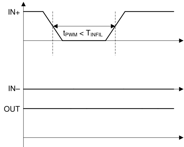
図 7-4. IN+ OFF Deglitch Filter
