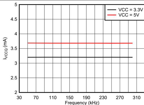
図 6-8. I_{VCCQ} Supply Current vs Input Frequency
