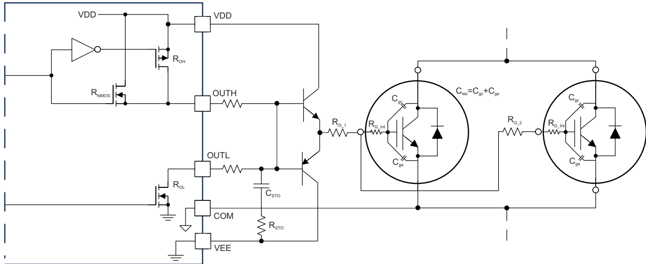
図 9-11. Current Buffer for Increased Drive Strength
