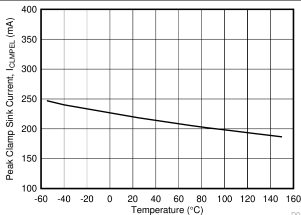
图 6-22. I_{CLMPEL} Miller Clamp Sink Current vs Temperature
