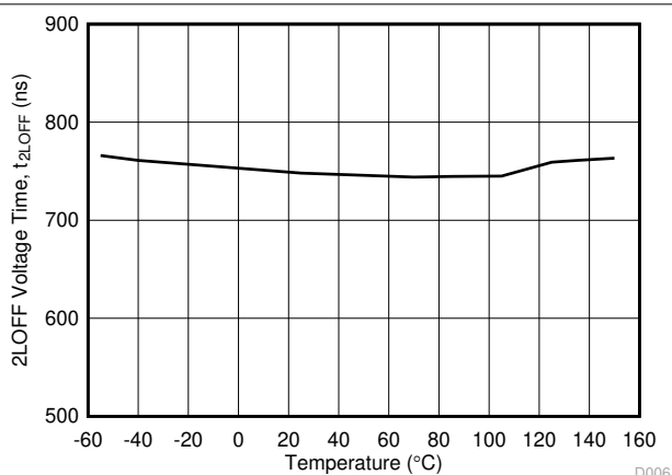
図 5-28. t_{2LOFF} 2-Level Turn Off Time vs Temperature
