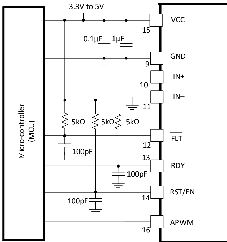
図 8-3. \overline{\text{FLT}} , \text{RDY} and \overline{\text{RST/EN}} Pins Circuitry
