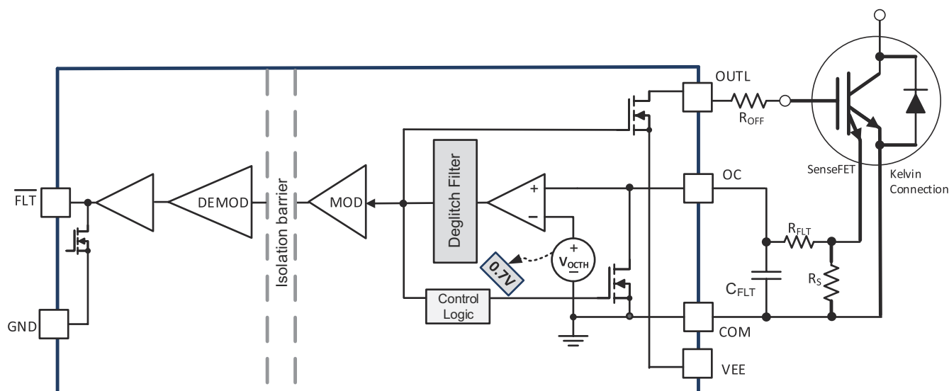
8-8. Overcurrent and Short Circuit Protection Based on IGBT Module with SenseFET
