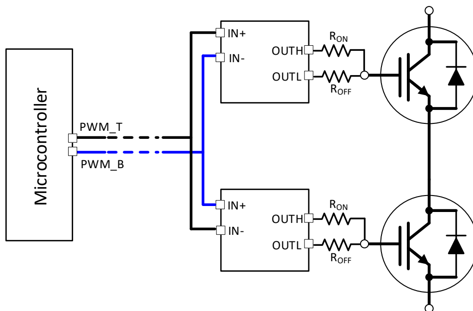
図 8-2. PWM Interlock for a Half Bridge
