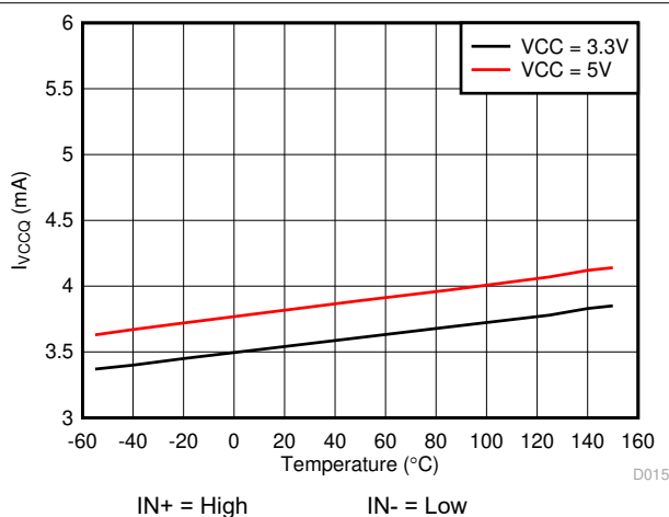
図 5-6. I_{VCCQ} Supply Current vs Temperature
