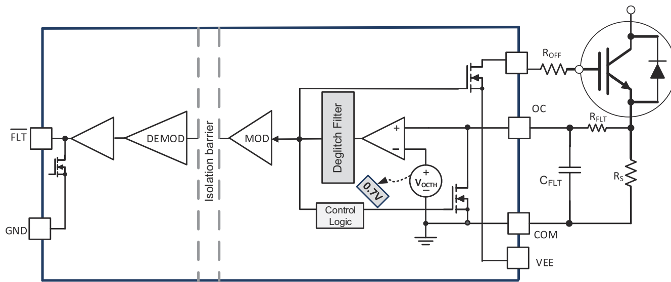
8-10. Overcurrent and Short Circuit Protection Based on Shunt Resistor
