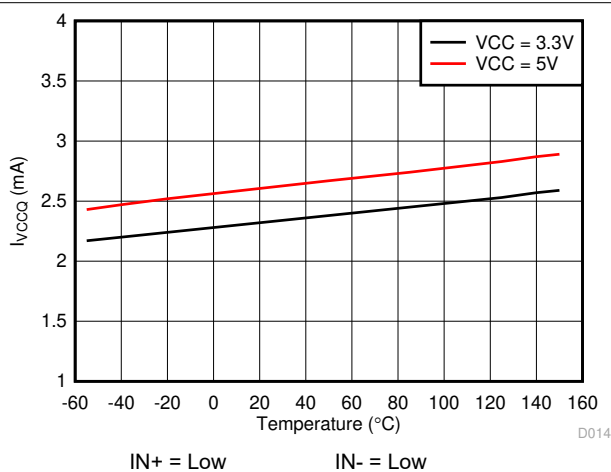
図 5-7. I_{VCCQ} Supply Current vs Temperature
