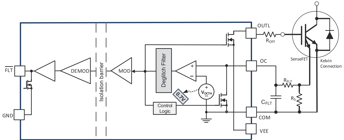
8-7. Overcurrent and Short Circuit Protection Based on IGBT Module with SenseFET
