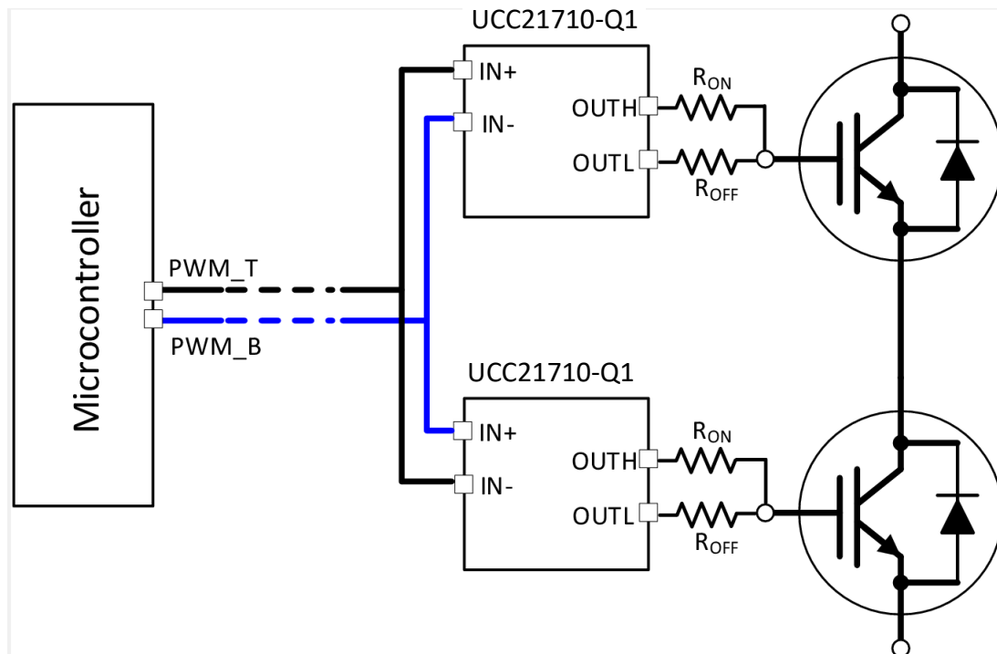
図 8-2. PWM Interlock for a Half Bridge
