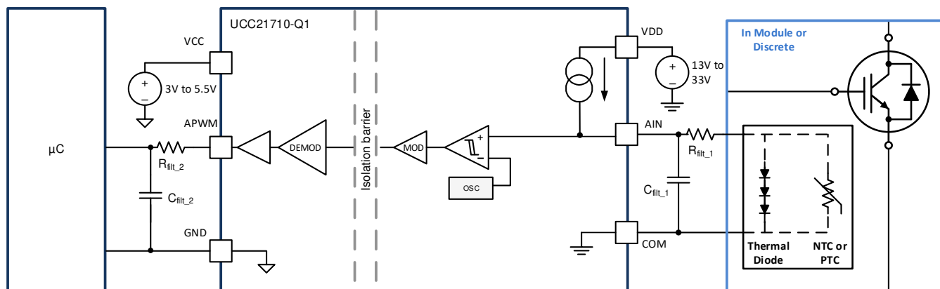
Figure 8-11. APWM Channel with Filtered Output
