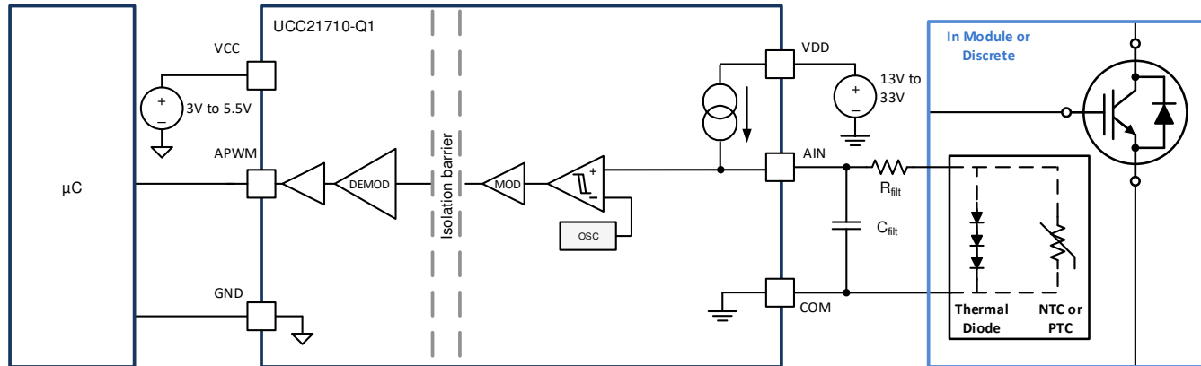
Figure 8-10. Thermal Diode or Thermistor Temperature Sensing Configuration
