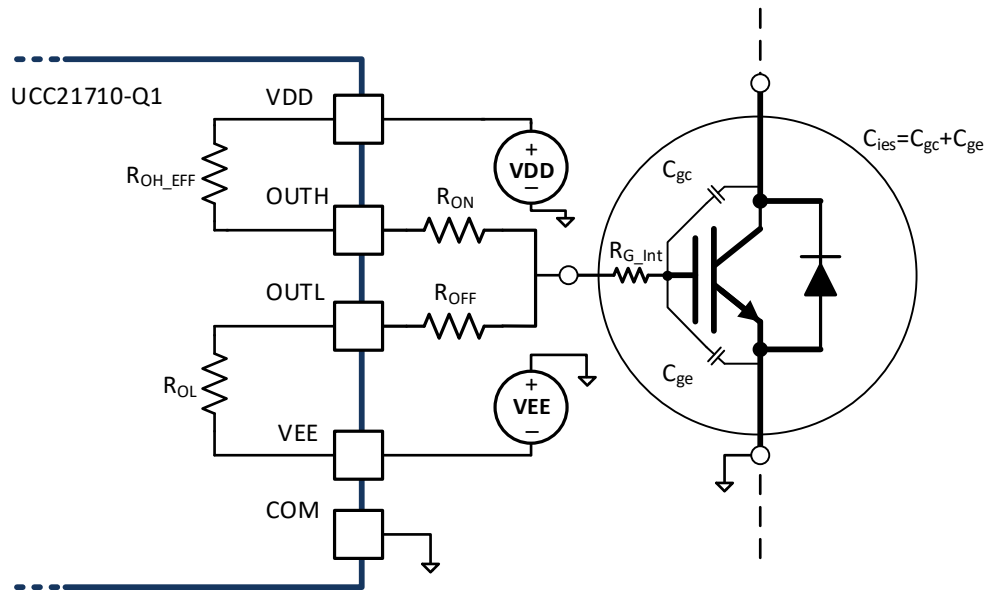
8-5. Output Model for Calculating Peak Gate Current
