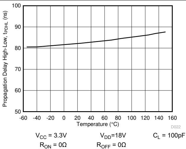
図 5-15. Propagation Delay t_{PDHL} vs. Temperature
