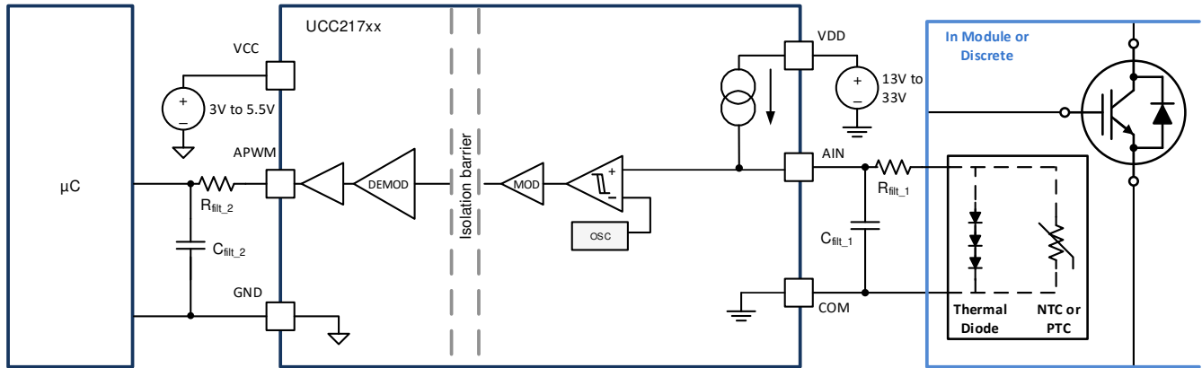
FIG 9-11. APWM Channel with Filtered Output
