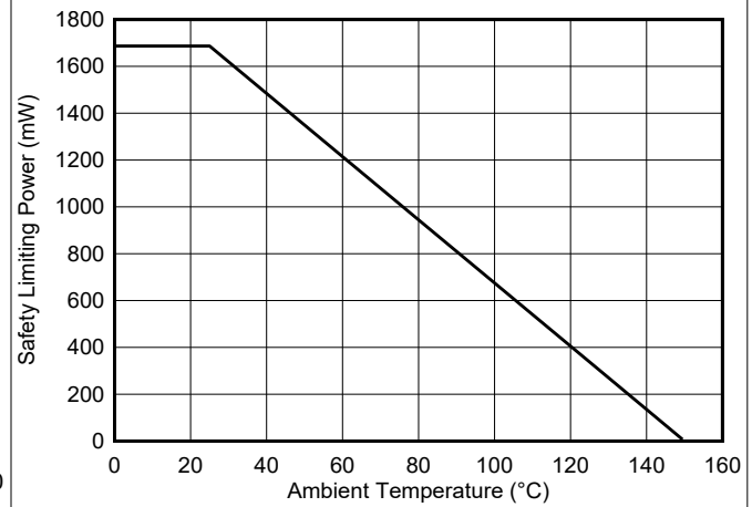
図 5-2. Thermal Derating Curve for Safety-Related Limiting Power per VDE
