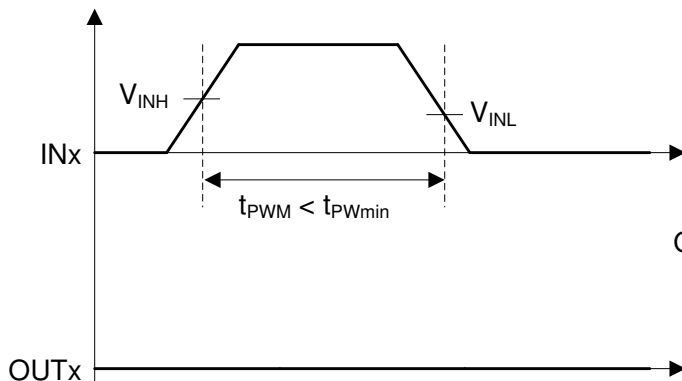
図 6-1. Deglitch Filter – Turn ON
