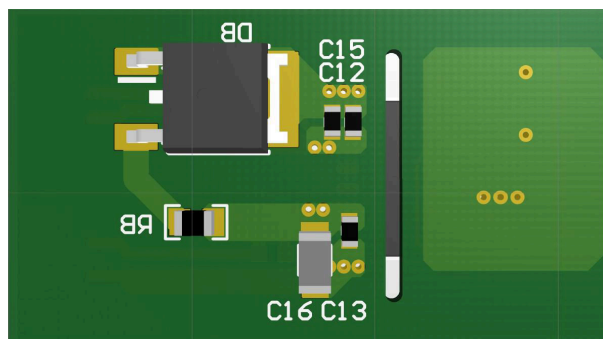
図 11-5. 3-D PCB Bottom View
