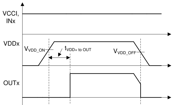
FIG 31. VDDA/B Power-up UVLO Delay
