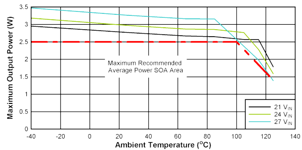
FIG 10-2. SOA Derating Curves: V_{DD-VEE} = 18\text{ V} , V_{COM-VEE} = 5\text{ V} , T_{shut}=160^\circ\text{C} , No Load on V_{COM-VEE} .
