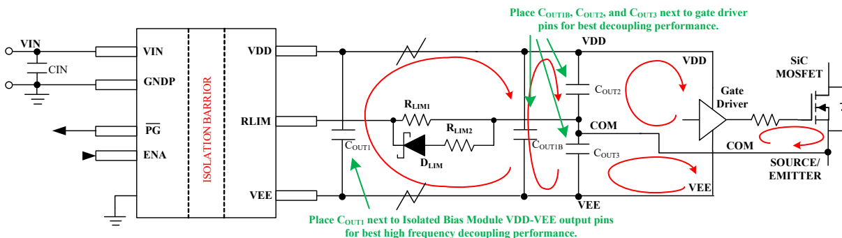
FIG 12-4. Dual Output Schematic with C_{out1} , C_{out1B} , C_{out2} , and C_{out3}
