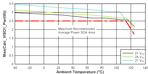
FIG 10-3. SOA Derating Curves: V_{DD-VEE} = 22\text{ V} , V_{COM-VEE} = 4\text{ V} , T_{shut}=160^\circ\text{C} , No Load on V_{COM-VEE} .
