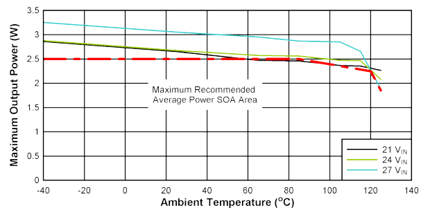
FIG 10-4. SOA Derating Curves: V_{DD-VEE} = 25\text{ V} , V_{COM-VEE} = 5\text{ V} , T_{shut}=160^\circ\text{C} , No Load on V_{COM-VEE} .
