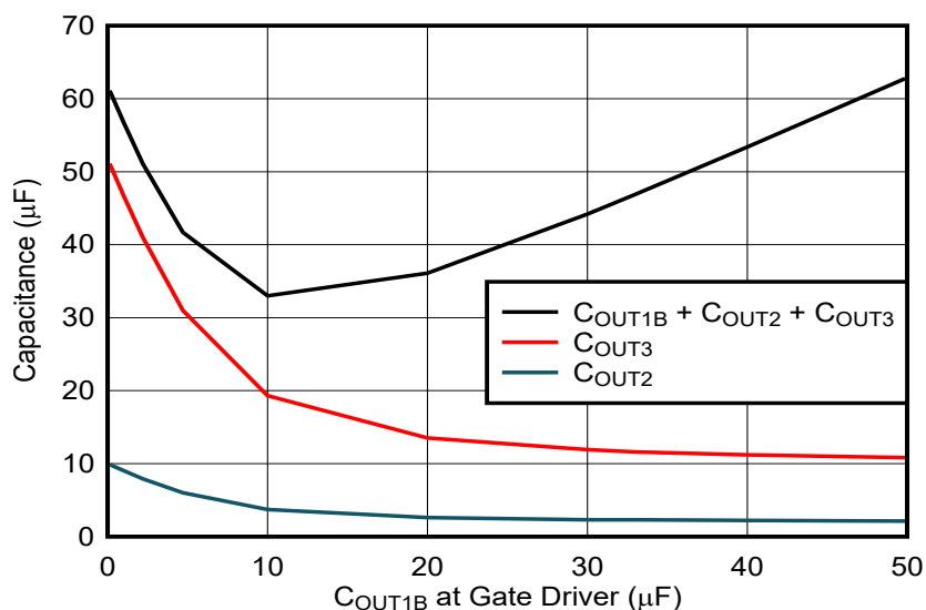
FIG 12-5. Output Capacitance variation with C_{out1B} selection
