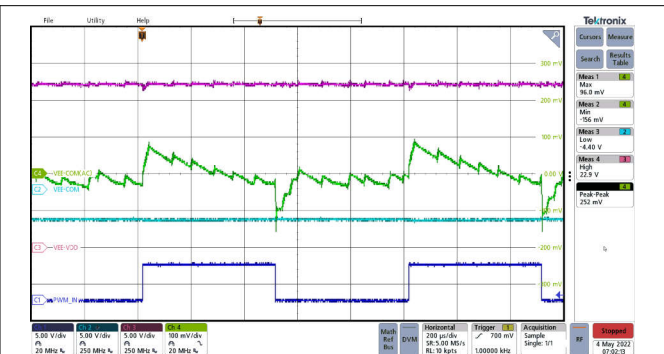
Figure 12-12. Ripple voltage: VEE-COM Switching 100-nF Load at 1 kHz.
