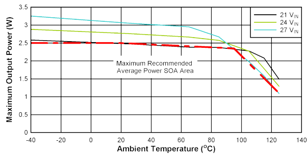
FIG 10-1. SOA Derating Curves: V_{DD-VEE} = 15\text{ V} , V_{COM-VEE} = 5\text{ V} , T_{shut}=160^\circ\text{C} , No Load on V_{COM-VEE} .
