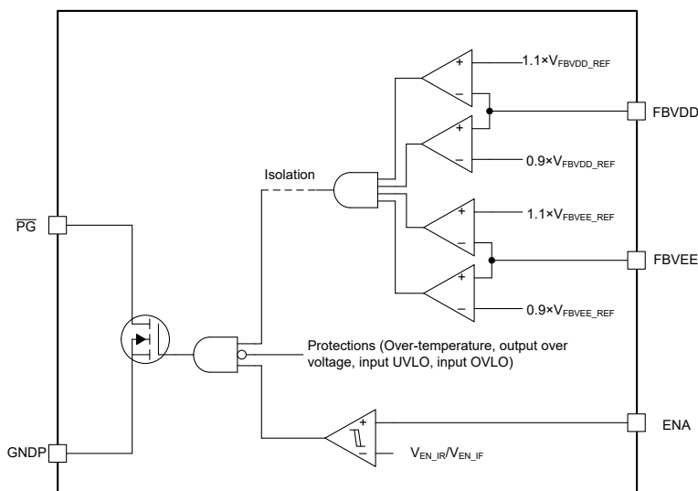
11-7. \overline{\text{PG}} Pin Logic
