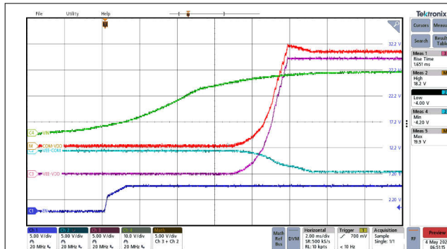
图 12-11. Power-Up Sequence.
