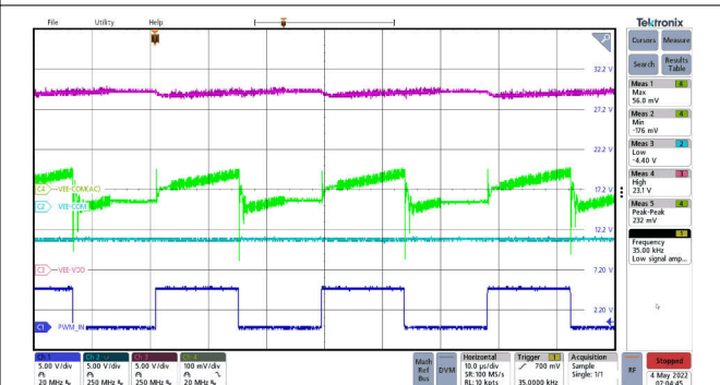
图 12-14. Ripple voltage: VEE-COM Switching 100-nF Load at 35 kHz.
