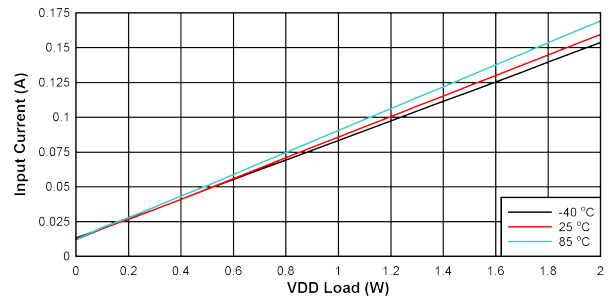
FIG 10-19. Input Current vs Load on V_{DD-VEE} : V_{IN} = 21\text{ V} , V_{DD-VEE} = 22\text{ V} , V_{COM-VEE} = 4\text{ V} , No Load on V_{COM-VEE}
