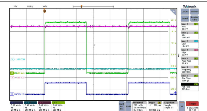
图 12-16. Gate Waveform Switching 100 nF at 1 kHz.
