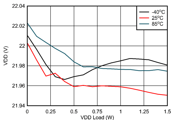
Figure 6-12. V_{D-D-VEE} Load Regulation: V_{IN} = 16.5V , V_{D-D-VEE} = 22V , V_{COM-VEE} = 4V
