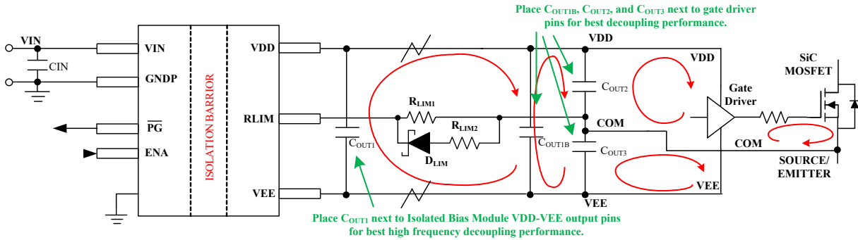
図 8-4. Dual Output Schematic with C_{out1} , C_{out1B} , C_{out2} , and C_{out3}
