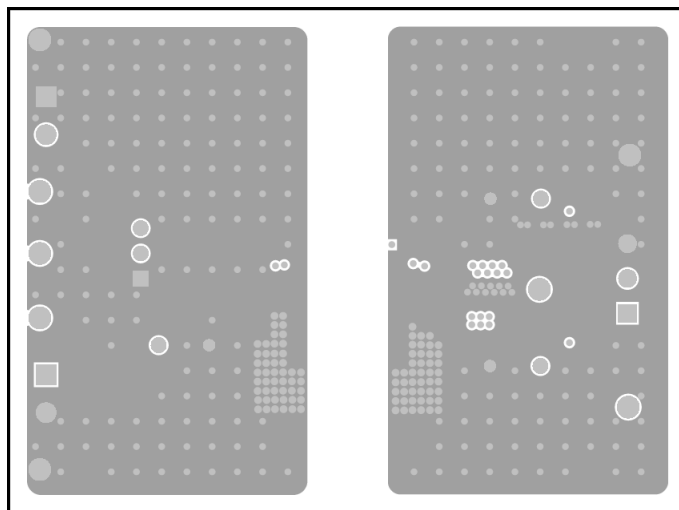
図 8-22. UCC14341-Q1EVM, Signal Layer 2 (Same as Layer 3)
