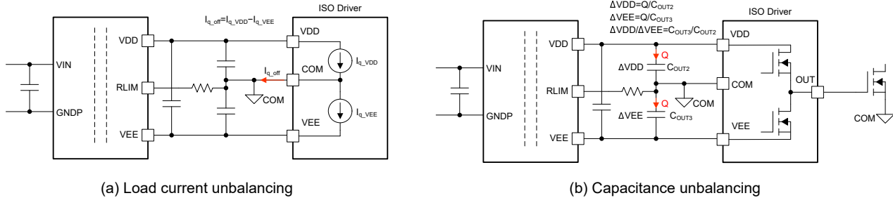
图 8-7. Source of Voltage Unbalancing
