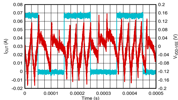
Figure 6-9. Load Transient Response: Between No Load and 1.5W, V_{IN} = 15V , V_{D-D-VEE} = 22V , V_{COM-VEE} = 4V
