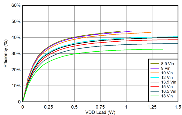
図 6-32. UCC14341B-Q1 Efficiency vs. Load on V_{DD-VEE} : T_{AMBIENT} = 85^{\circ}\text{C} , V_{DD-VEE} = 15\text{V} , V_{COM-VEE} = 4\text{V} , No Load on V_{COM-VEE}
