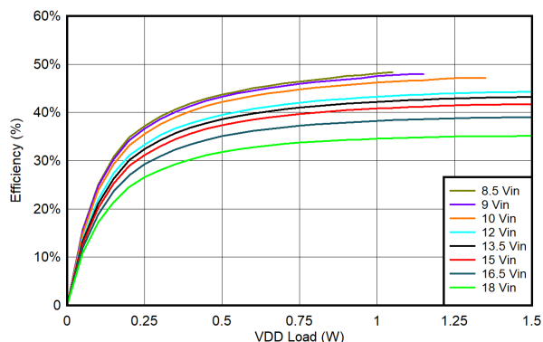
FIG 6-31. UCC14341B-Q1 Efficiency vs. Load on V_{DD-VEE} : T_{AMBIENT} = 25^{\circ}C , V_{DD-VEE} = 15V , V_{COM-VEE} = 4V , No Load on V_{COM-VEE}
