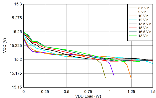
FIG 6-29. UCC14341B-Q1 V_{DD-VEE} Load Regulation: T_{AMBIENT} = 85^{\circ}C , V_{DD-VEE} = 15V , V_{COM-VEE} = 4V
