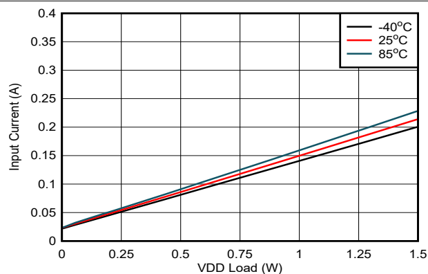
図 6-22. Input Current vs. Load on V_{DD-VEE} : V_{IN} = 13.5V , V_{DD-VEE} = 22V , V_{COM-VEE} = 4V , No Load on V_{COM-VEE}
