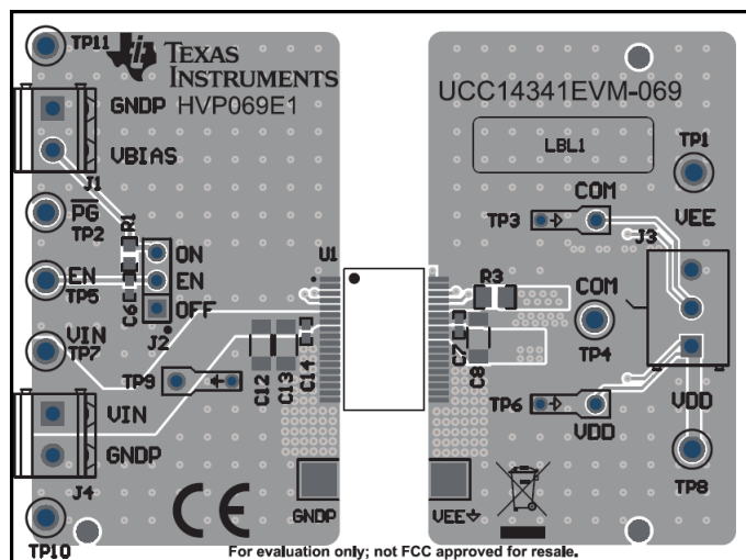
図 8-21. UCC14341-Q1EVM, PCB Top Layer, Assembly
