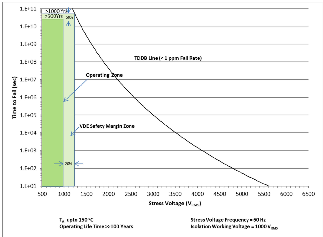
図 6-1. TDDB: Insulation Lifetime Projection for 1000 Vrms Working Voltage.
