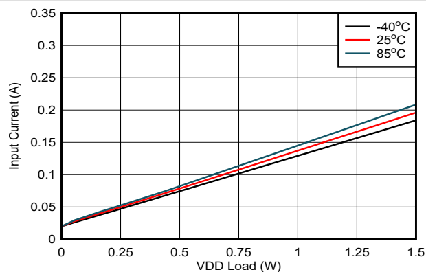
図 6-23. Input Current vs. Load on V_{DD-VEE} : V_{IN} = 15V , V_{DD-VEE} = 22V , V_{COM-VEE} = 4V , No Load on V_{COM-VEE}
