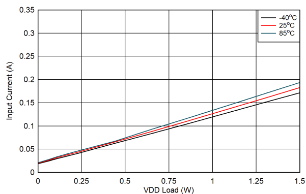
図 6-25. Input Current vs. Load on V_{DD-VEE} : V_{IN} = 18V , V_{DD-VEE} = 22V , V_{COM-VEE} = 4V , No Load on V_{COM-VEE}
