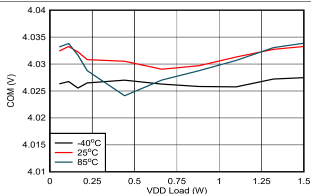
FIG 6-16. V_{COM-VEE} Load Regulation: V_{IN} = 16.5V , V_{VDD-VEE} = 22V , V_{COM-VEE} = 4V
