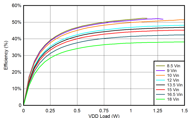
FIG 6-30. UCC14341B-Q1 Efficiency vs. Load on V_{DD-VEE} : T_{AMBIENT} = -40^{\circ}C , V_{DD-VEE} = 15V , V_{COM-VEE} = 4V , No Load on V_{COM-VEE}
