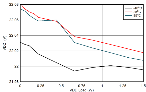
Figure 6-13. V_{VDD-VEE} Load Regulation: V_{IN} = 18V , V_{VDD-VEE} = 22V , V_{COM-VEE} = 4V
