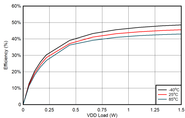
図 6-21. Efficiency vs. Load on V_{DD-VEE} : V_{IN} = 18V , V_{DD-VEE} = 22V , V_{COM-VEE} = 4V , No Load on V_{COM-VEE}
