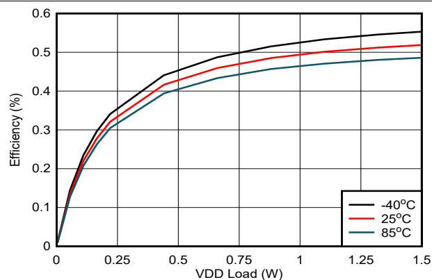
FIG 6-18. Efficiency vs. Load on V_{VDD-VEE} : V_{IN} = 13.5V , V_{VDD-VEE} = 22V , V_{COM-VEE} = 4V , No Load on V_{COM-VEE}
