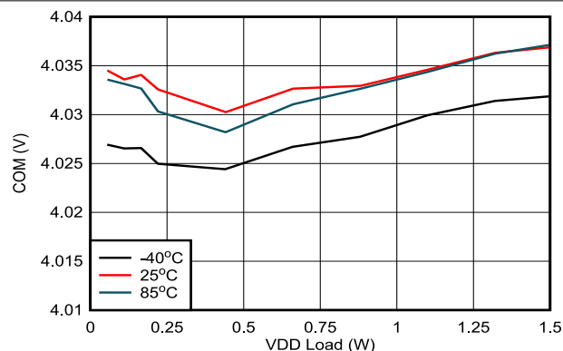
FIG 6-14. V_{COM-VEE} Load Regulation: V_{IN} = 13.5V , V_{VDD-VEE} = 22V , V_{COM-VEE} = 4V
