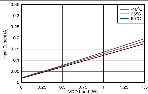
図 6-24. Input Current vs. Load on V_{DD-VEE} : V_{IN} = 16.5V , V_{DD-VEE} = 22V , V_{COM-VEE} = 4V , No Load on V_{COM-VEE}
