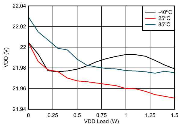
Figure 6-11. V_{VDD-VEE} Load Regulation: V_{IN} = 15V , V_{VDD-VEE} = 22V , V_{COM-VEE} = 4V
