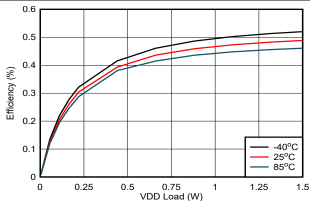
図 6-20. Efficiency vs. Load on V_{DD-VEE} : V_{IN} = 16.5V , V_{DD-VEE} = 22V , V_{COM-VEE} = 4V , No Load on V_{COM-VEE}
