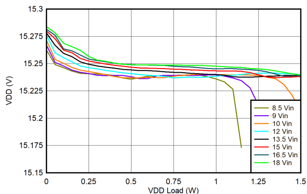
FIG 6-27. UCC14341B-Q1 V_{DD-VEE} Load Regulation: T_{AMBIENT} = -40^{\circ}C , V_{DD-VEE} = 15V , V_{COM-VEE} = 4V
