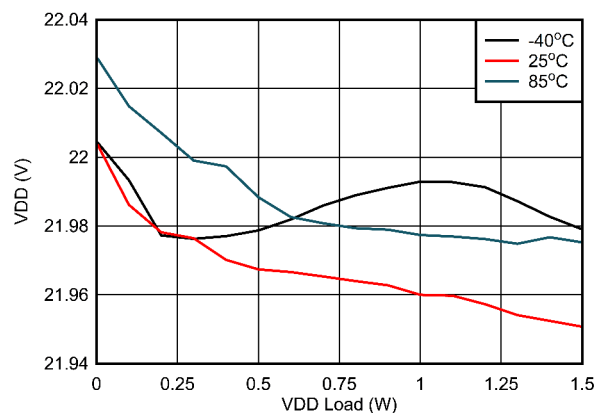
Figure 6-11. V_{D-D-VEE} Load Regulation: V_{IN} = 15V , V_{D-D-VEE} = 22V , V_{COM-VEE} = 4V
