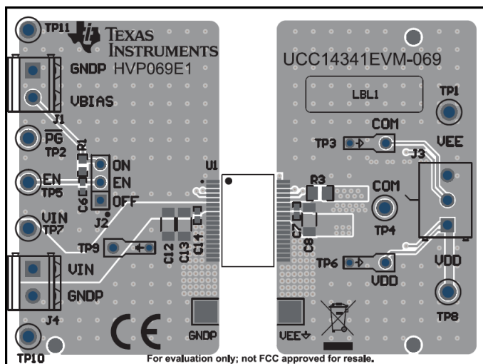
8-21. UCC14341-Q1EVM, PCB Top Layer, Assembly
