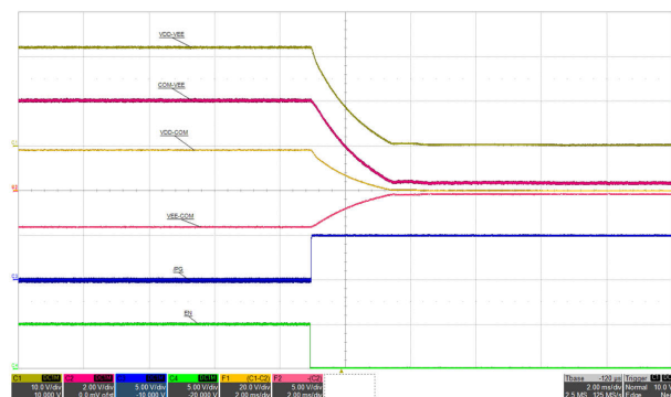
Figure 6-8. Shutdown: V_{IN} = 15V , V_{VDD-VEE} = 22V , V_{COM-VEE} = 4V , I_{VDD-VEE} = 68mA , No Load on V_{COM-VEE} . Time Scale: 2ms/div.
