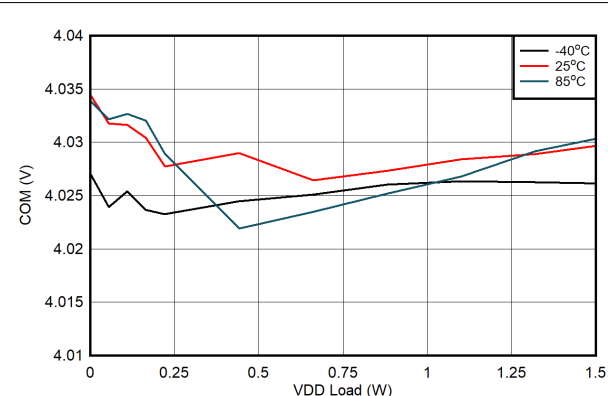
FIG 6-17. V_{COM-VEE} Load Regulation: V_{IN} = 18V , V_{VDD-VEE} = 22V , V_{COM-VEE} = 4V
