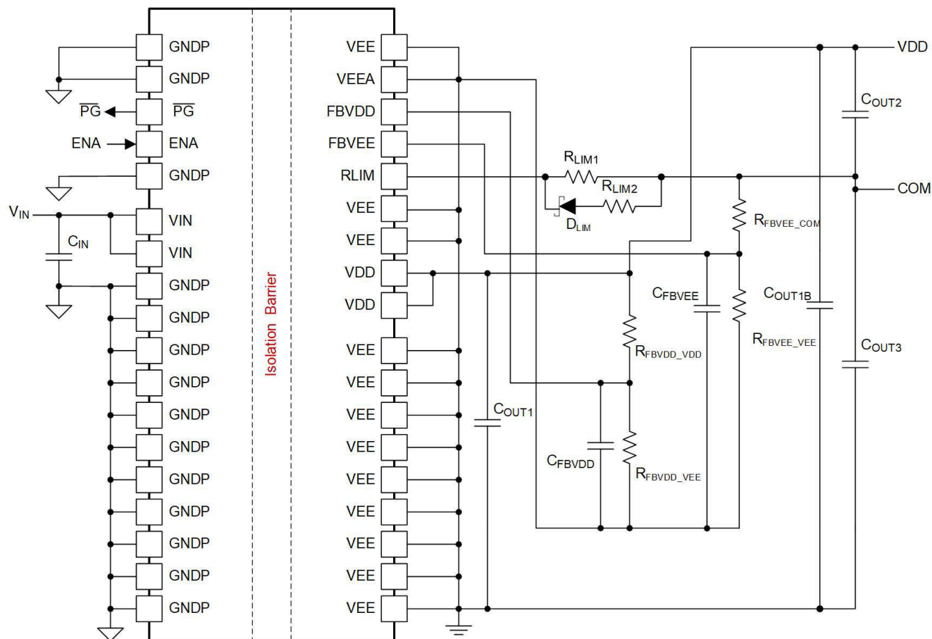
図 8-8. Dual output application schematic configured for V_{COM\_VEE} regulation > 2.5V
