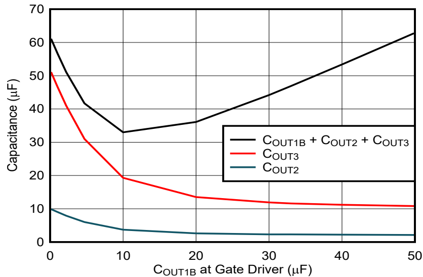
図 8-5. Output Capacitance Variation with C_{out1B} selection
