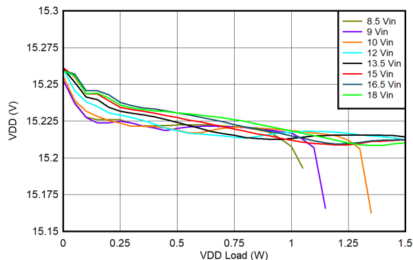
FIG 6-28. UCC14341B-Q1 V_{DD-VEE} Load Regulation: T_{AMBIENT} = 25^{\circ}C , V_{DD-VEE} = 15V , V_{COM-VEE} = 4V
