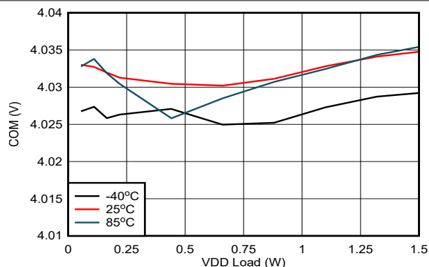
FIG 6-15. V_{COM-VEE} Load Regulation: V_{IN} = 15V , V_{VDD-VEE} = 22V , V_{COM-VEE} = 4V
