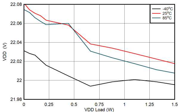
Figure 6-13. V_{D-D-VEE} Load Regulation: V_{IN} = 18V , V_{D-D-VEE} = 22V , V_{COM-VEE} = 4V
