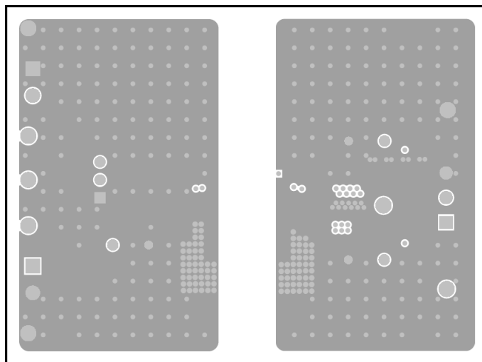
8-22. UCC14341-Q1EVM, Signal Layer 2 (Same as Layer 3)
