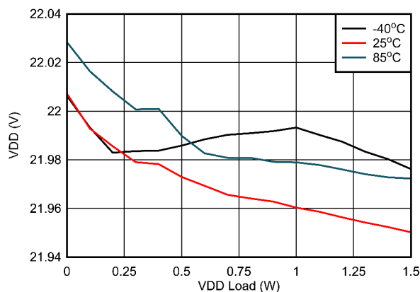
Figure 6-10. V_{D-D-VEE} Load Regulation: V_{IN} = 13.5V , V_{D-D-VEE} = 22V , V_{COM-VEE} = 4V
