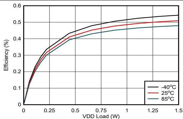
FIG 6-19. Efficiency vs. Load on V_{VDD-VEE} : V_{IN} = 15V , V_{VDD-VEE} = 22V , V_{COM-VEE} = 4V , No Load on V_{COM-VEE}
