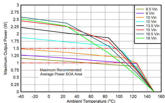
FIG 6-26. UCC14341B-Q1 SOA Derating Curves: V_{DD-VEE} = 15V , V_{COM-VEE} = 5V , T_{shut}=160^{\circ}C , No Load on V_{COM-VEE}
