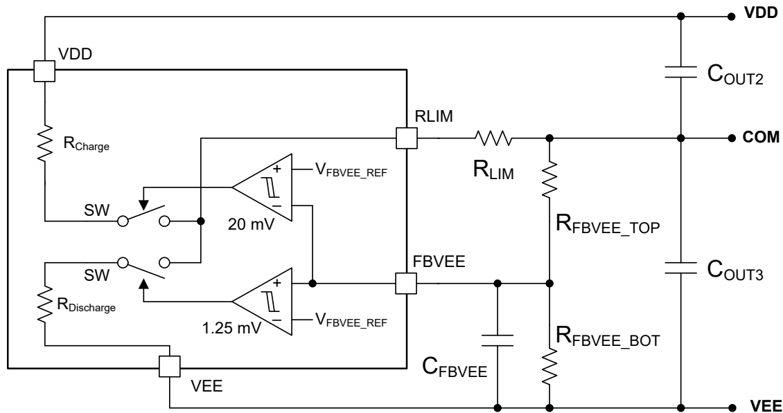
図 8-2. COM-VEE Voltage Regulation
