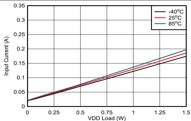
図 7-20. Input Current vs. Load on V_{DD-VEE} : V_{IN} = 16.5\text{ V} , V_{DD-VEE} = 22\text{ V} , V_{COM-VEE} = 4\text{ V} , No Load on V_{COM-VEE}
