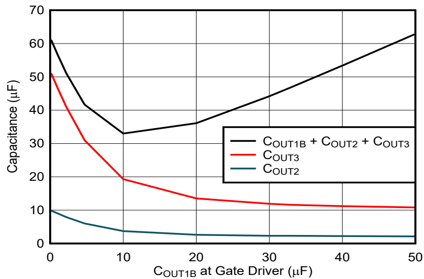
图 9-5. Output Capacitance variation with C_{OUT1B} selection
