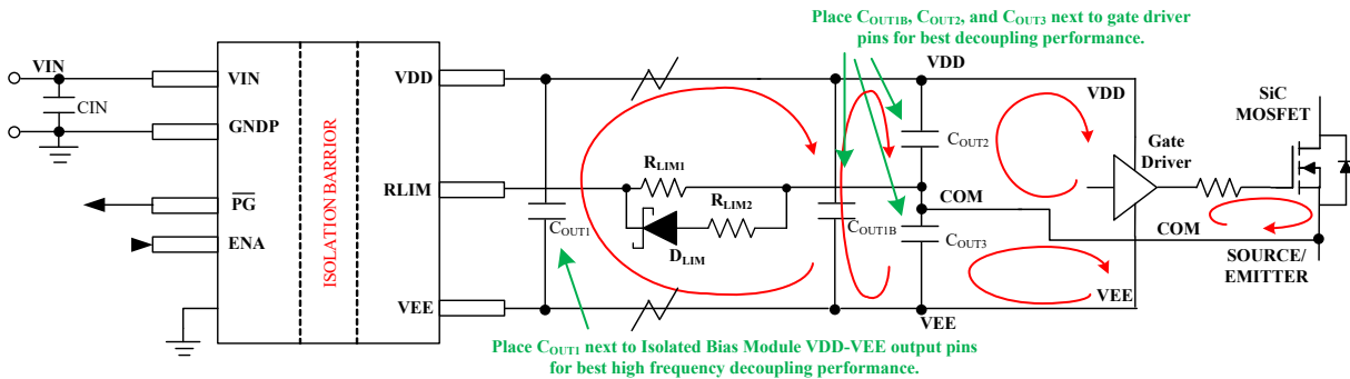
图 9-4. Dual Output Schematic with C_{OUT1} , C_{OUT1B} , C_{OUT2} , and C_{OUT3}
