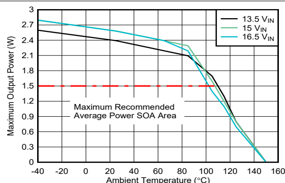
図 7-5. SOA Derating Curves: V_{DD-VEE} = 22\text{ V} , V_{COM-VEE} = 4\text{ V} , T_{shut}=150^\circ\text{C} , No Load on V_{COM-VEE} , tested in a shielded box.
