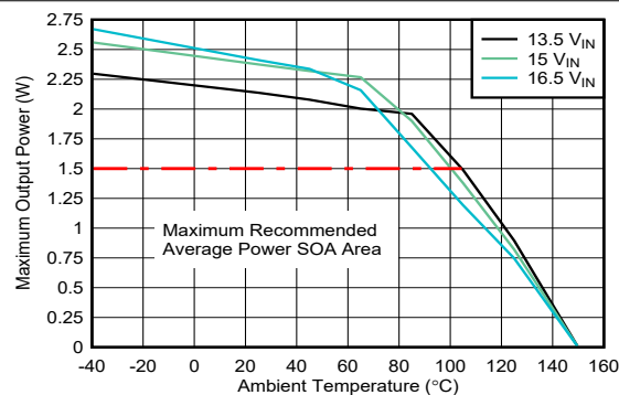
図 7-3. SOA Derating Curves: V_{DD-VEE} = 22\text{ V} , V_{COM-VEE} = 4\text{ V} , T_{shut}=160^\circ\text{C} , No Load on V_{COM-VEE}
