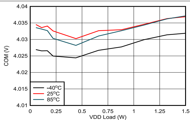
図 7-12. V_{COM-VEE} Load Regulation: V_{IN} = 13.5\text{ V} , V_{VDD-VEE} = 22\text{ V} , V_{COM-VEE} = 4\text{ V}
