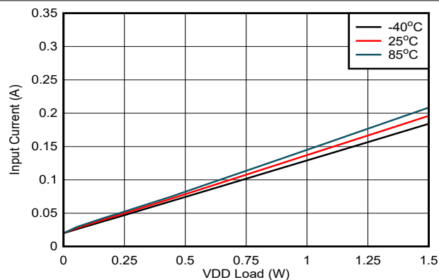
図 7-19. Input Current vs. Load on V_{DD-VEE} : V_{IN} = 15\text{ V} , V_{DD-VEE} = 22\text{ V} , V_{COM-VEE} = 4\text{ V} , No Load on V_{COM-VEE}
