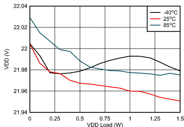
Figure 7-10. V_{VDD-VEE} Load Regulation: V_{IN} = 15\text{ V} , V_{VDD-VEE} = 22\text{ V} , V_{COM-VEE} = 4\text{ V}
