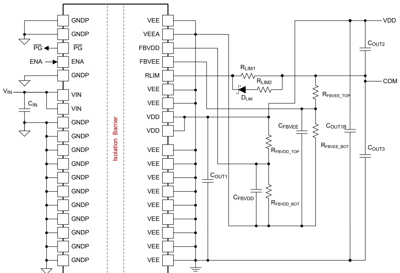
図 9-1. Dual Adjustable Output Configuration
