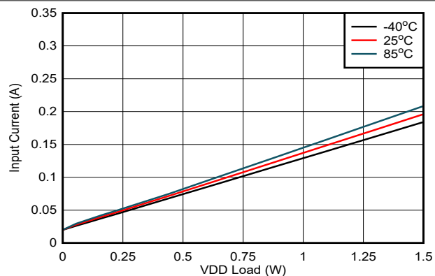
FIG 7-19. Input Current vs. Load on V_{DD-VEE} : V_{IN} = 15\text{ V} , V_{DD-VEE} = 22\text{ V} , V_{COM-VEE} = 4\text{ V} , No Load on V_{COM-VEE}
