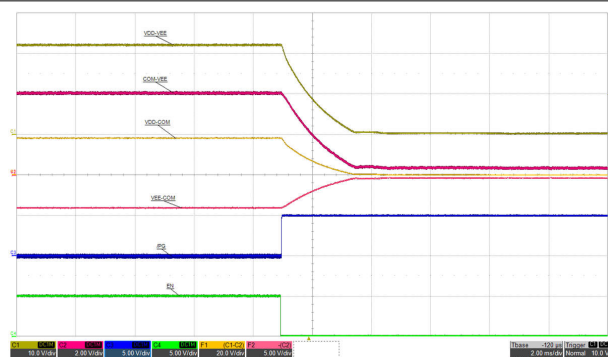
図 7-7. Shutdown: V_{IN} = 15\text{ V} , V_{VDD-VEE} = 22\text{ V} , V_{COM-VEE} = 4\text{ V} , I_{VDD-VEE} = 68\text{ mA} , No Load on V_{COM-VEE} . Time Scale: 2ms/div.
