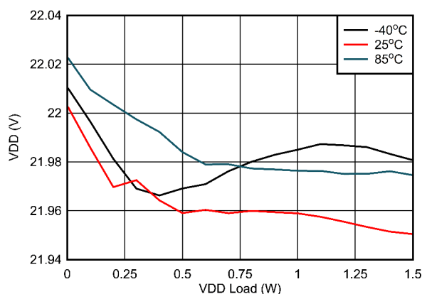
図 7-11. V_{VDD-VEE} Load Regulation: V_{IN} = 16.5\text{ V} , V_{VDD-VEE} = 22\text{ V} , V_{COM-VEE} = 4\text{ V}
