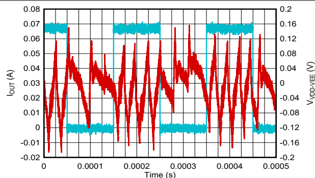
Figure 7-8. Load Transient Response: Between No Load and 1.5W, V_{IN} = 15\text{ V} , V_{VDD-VEE} = 22\text{ V} , V_{COM-VEE} = 4\text{ V}
