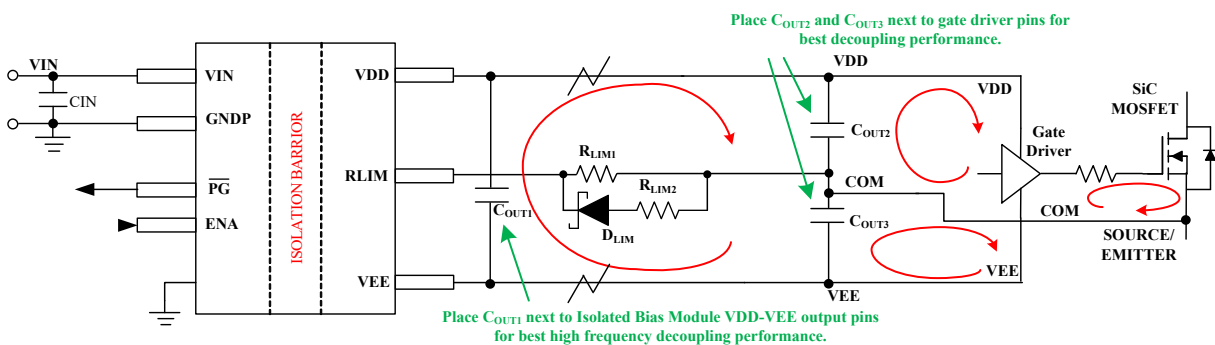
図 9-3. Dual Output Schematic with C_{OUT1} , C_{OUT2} , and C_{OUT3}
