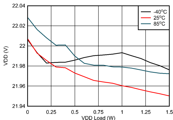
図 7-9. V_{VDD-VEE} Load Regulation: V_{IN} = 13.5\text{ V} , V_{VDD-VEE} = 22\text{ V} , V_{COM-VEE} = 4\text{ V}
