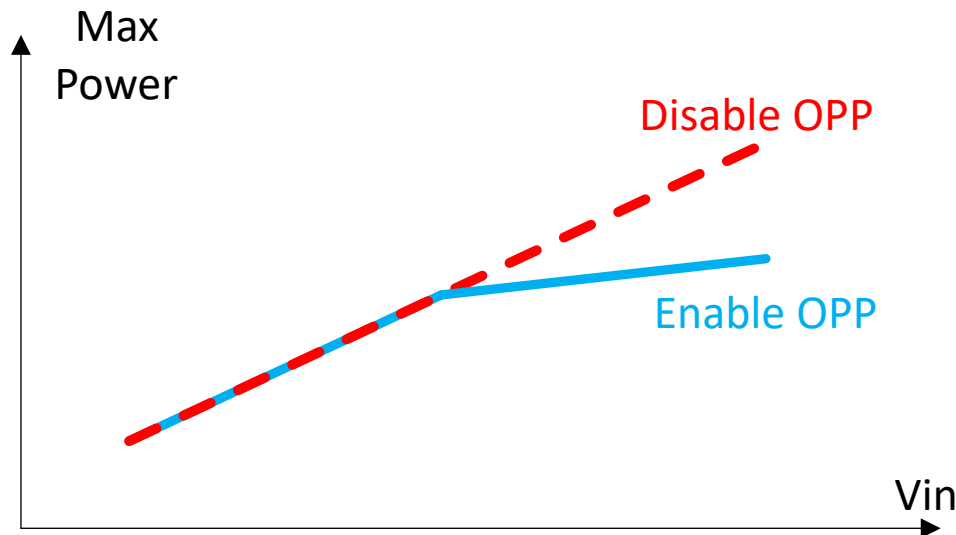
図 8-8. Maximum Output Power Under Different Input Voltage Condition
