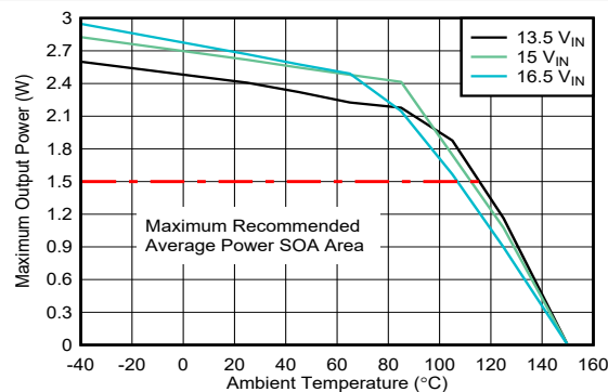
図 7-1. SOA Derating Curves: V_{DD-VEE} = 15\text{ V} , V_{COM-VEE} = 5\text{ V} , T_{shut}=160^\circ\text{C} , No Load on V_{COM-VEE}
