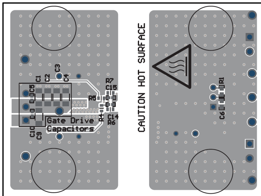
12-31. UCC14240EVM-052EVM, PCB Bottom Layer, Assembly (Mirrored View)
