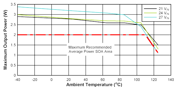
FIG 10-3. SOA Derating Curves: V_{DD-VEE} = 22\text{ V} , V_{COM-VEE} = 4\text{ V} , T_{shut}=150^\circ\text{C} , No Load on V_{COM-VEE} .
