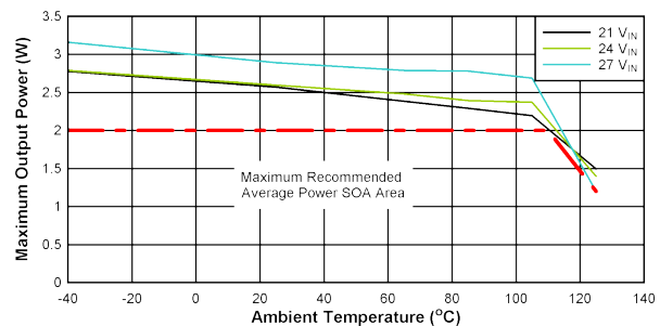
FIG 10-4. SOA Derating Curves: V_{DD-VEE} = 25\text{ V} , V_{COM-VEE} = 5\text{ V} , T_{shut}=150^\circ\text{C} , No Load on V_{COM-VEE} .
