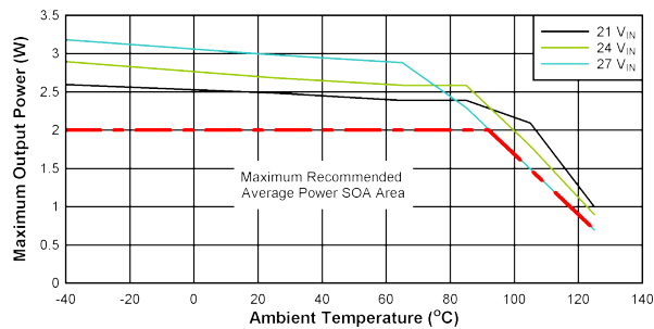
FIG 10-1. SOA Derating Curves: V_{DD-VEE} = 15\text{ V} , V_{COM-VEE} = 5\text{ V} , T_{shut}=150^\circ\text{C} , No Load on V_{COM-VEE} .
