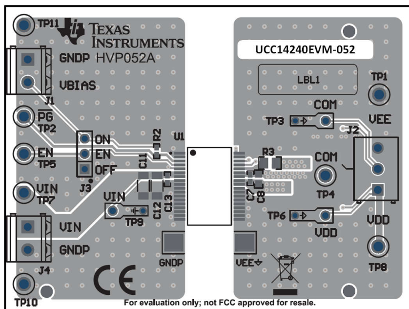
图 12-28. UCC14240EVM-052EVM, PCB Top Layer, Assembly (same EVM used as UCC14240-Q1)
