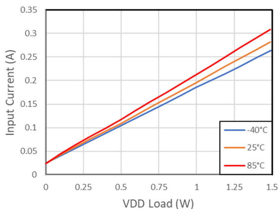
FIG 7-20. Input Current vs. Load on V_{DD-VEE} : V_{IN} = 12\text{ V} , V_{DD-VEE} = 22\text{ V} , V_{COM-VEE} = 4\text{ V} , No Load on V_{COM-VEE}
