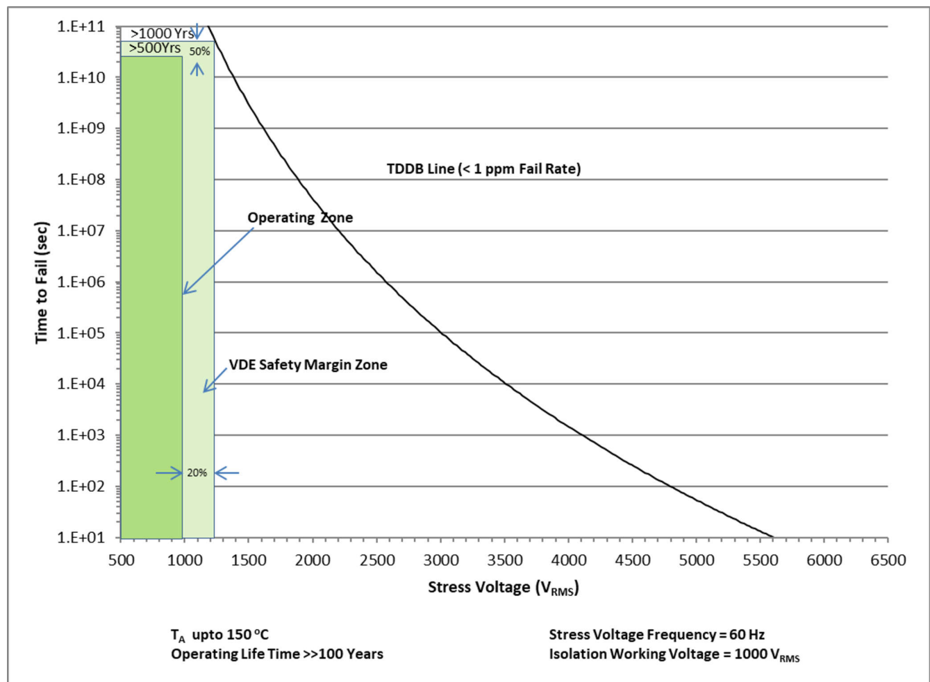
FIG 7-1. TDDB: Insulation Lifetime Projection for 1000 V_{RMS} Working Voltage.
