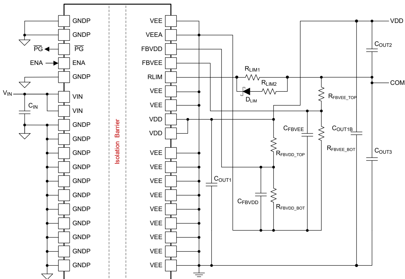
图 9-1. Dual Adjustable Output Configuration
