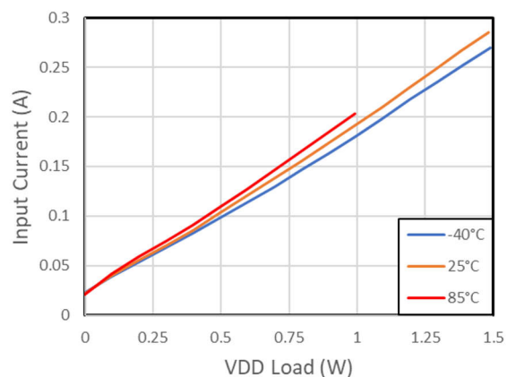
FIG 7-21. Input Current vs. Load on V_{DD-VEE} : V_{IN} = 18\text{ V} , V_{DD-VEE} = 22\text{ V} , V_{COM-VEE} = 4\text{ V} , No Load on V_{COM-VEE}
