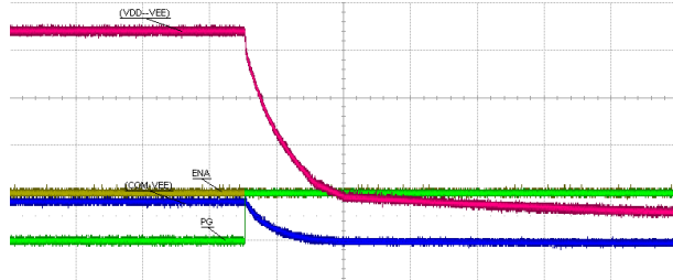
FIG 7-8. Shutdown: V_{IN} = 12\text{ V} , V_{VDD-VEE} = 22\text{ V} , V_{COM-VEE} = 4\text{ V} , No Load on V_{COM-VEE} . Voltage Scale: 5V/div, Time Scale: 50ms/div.
