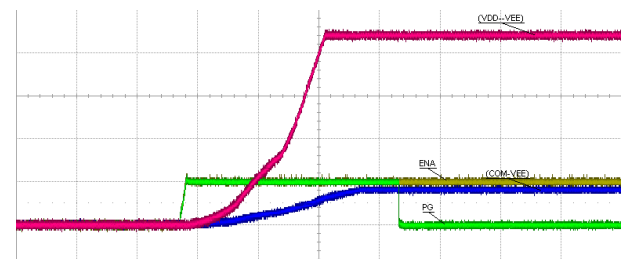
Figure 7-7. Start-up: V_{IN} = 12\text{ V} , V_{DD-VEE} = 22\text{ V} , V_{COM-VEE} = 4\text{ V} , No Load on V_{COM-VEE} . Voltage Scale: 5V/div, Time Scale: 2ms/div.
