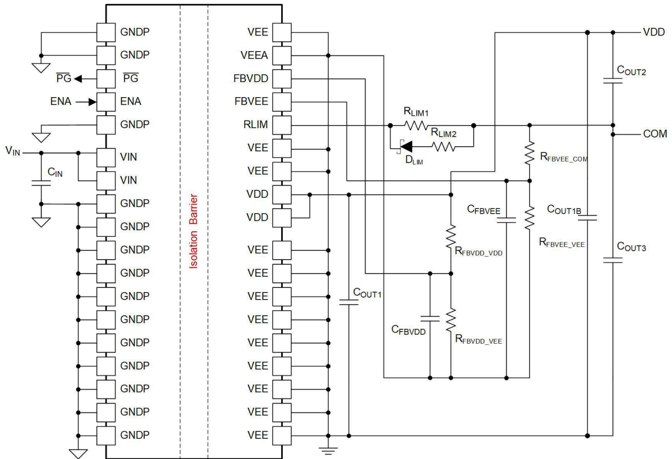
FIG 12-8. Dual output application schematic configured for \text{V}_{\text{COM\_VEE}} regulation > 2.5V
