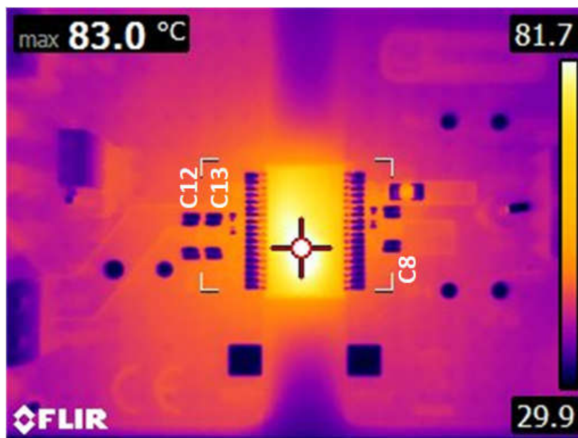
FIG 12-18. Thermal Image
