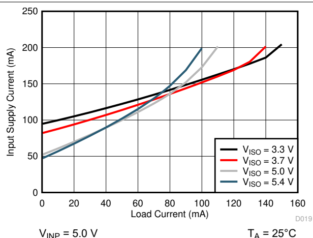
FIG 6-25. Input Supply Current ( I_{VINP} ) vs Load Current ( I_{ISO} )
