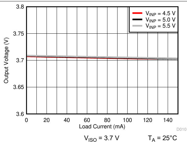
6-19. Isolated Supply Voltage ( V_{ISO} ) vs Load Current ( I_{ISO} )
