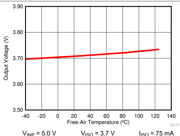
FIG 6-23. Isolated Supply Voltage ( V_{ISO} ) vs Free-Air Temperature
