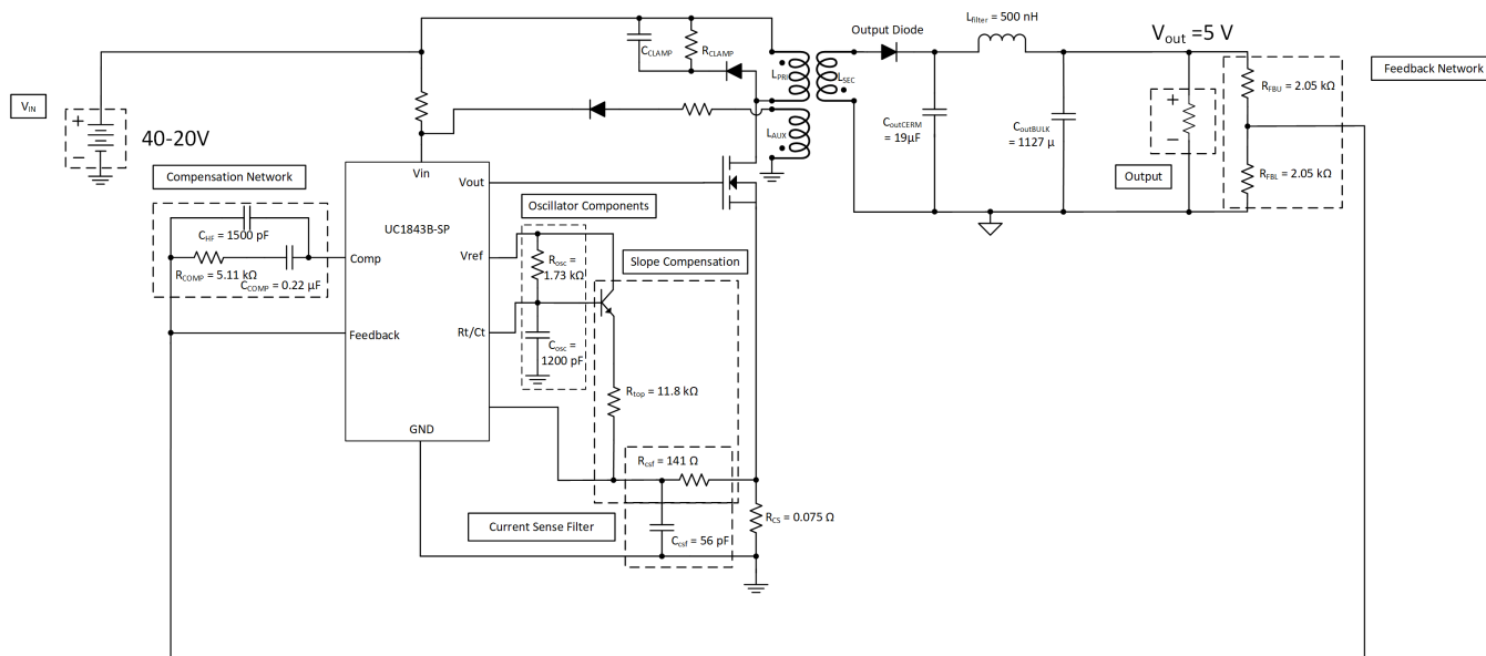
Figure 15. Flyback Regulator
