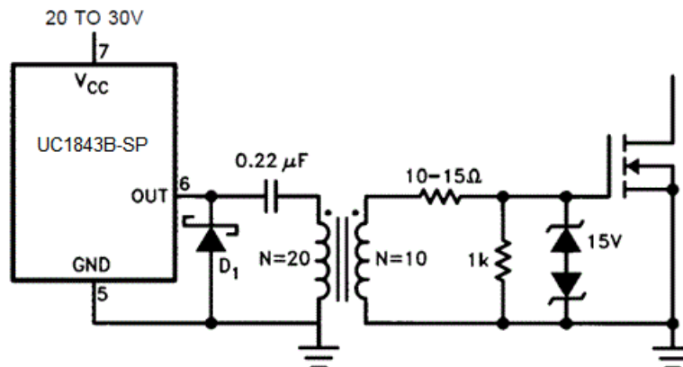
Figure 8. Direct MOSFET Drive
