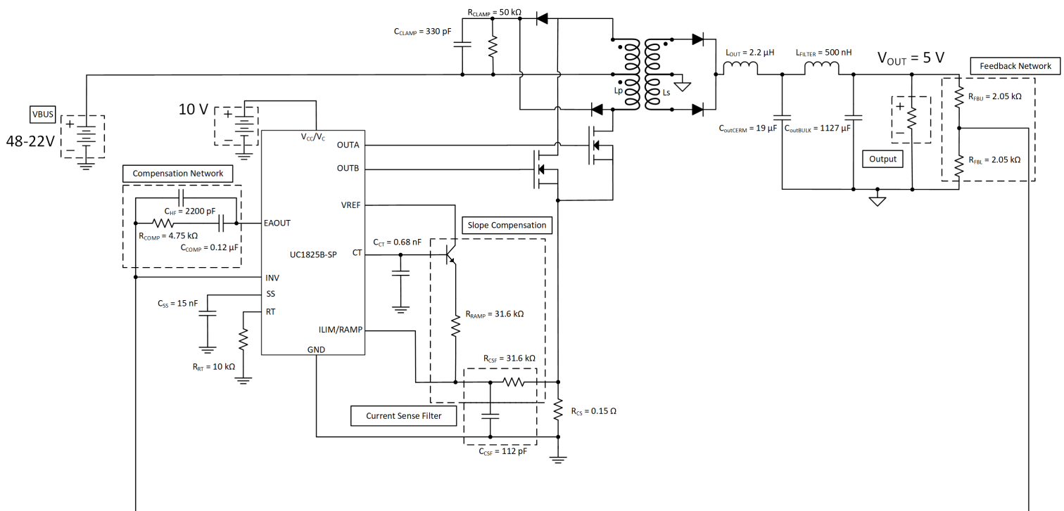
8-4. Typical Application
