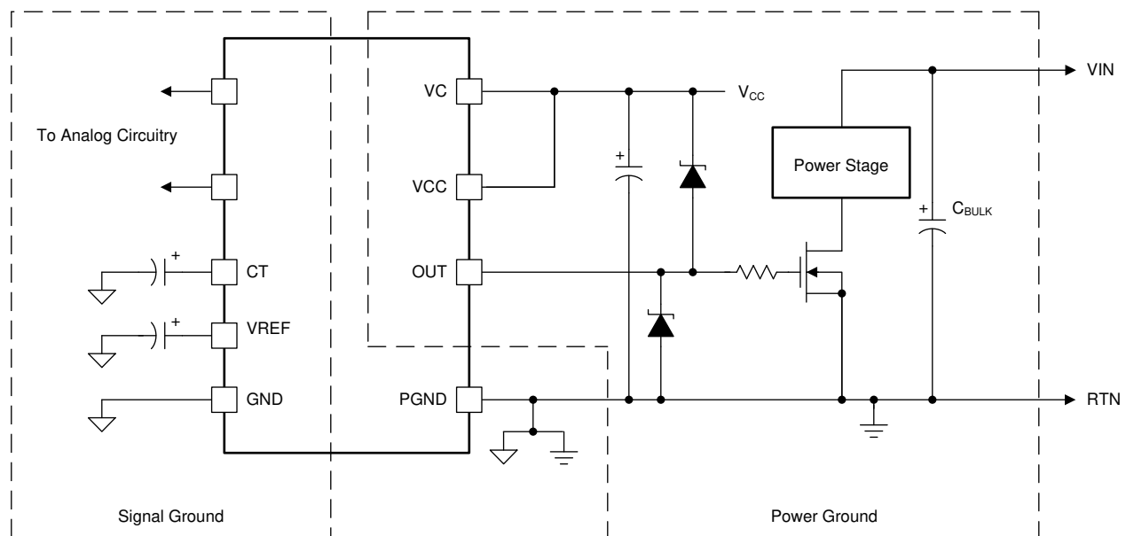
Figure 10-1. Ground Planes Diagram
