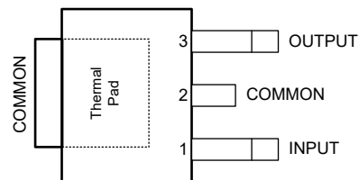
4-2. KVU Package, 3-Pin TO-252 (Top View)
