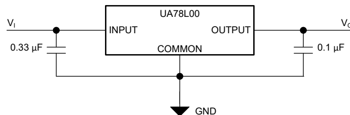
8-1. Fixed-Output Regulator
