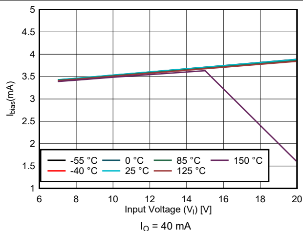
6-16. Bias Current vs Input Voltage for New Chip
