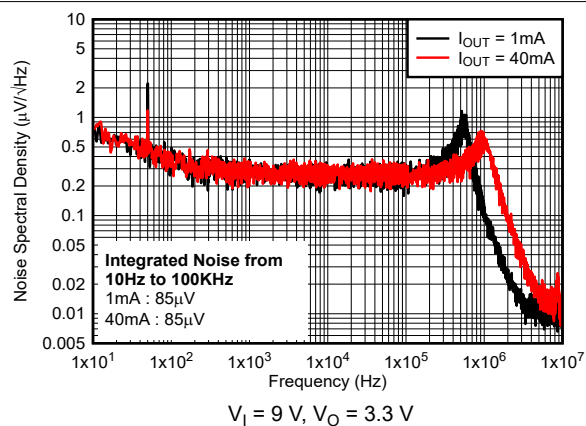
6-20. Noise Spectral Density vs Frequency and I_O for New Chip
