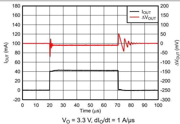
8-8. Load Transient Behavior for New Chip
