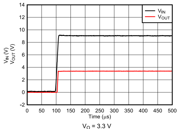
8-6. Start-Up With Fast V_I Ramp for New Chip
