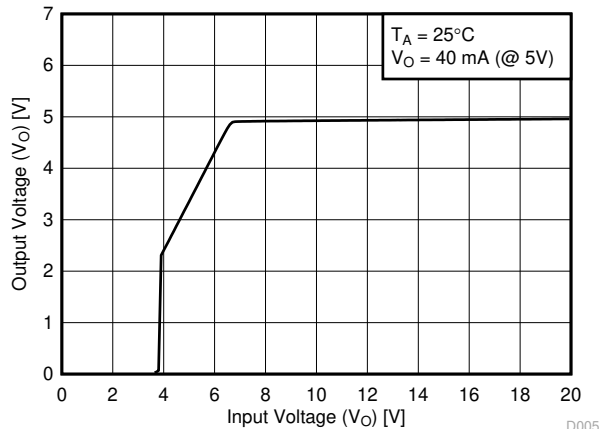
8-4. Output Voltage vs Input Voltage for Legacy Chip
