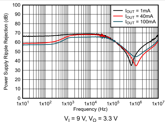
6-22. PSRR vs Frequency and I_O for New Chip
