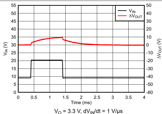
8-9. Line Transient Behavior for New Chip
