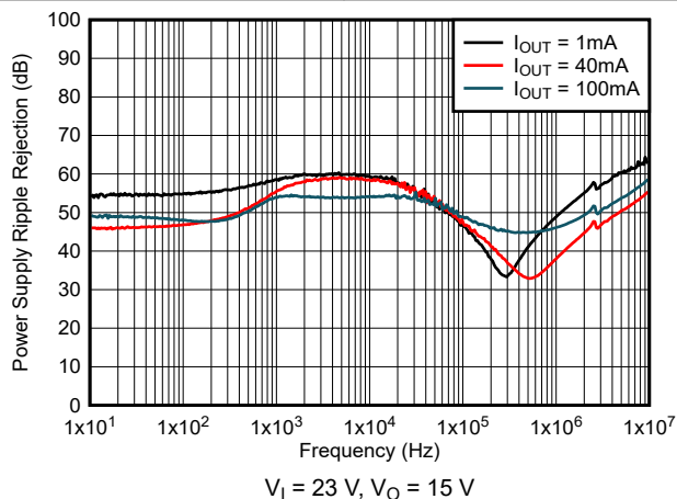
6-23. PSRR vs Frequency and I_O for New Chip
