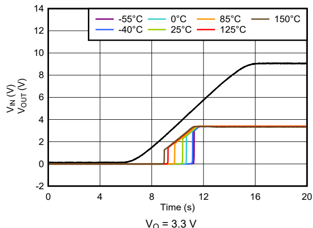
8-7. Start-Up With Slow V_I Ramp Across Temperature for New Chip
