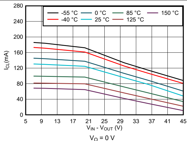
6-18. I_{SC} vs V_I for New Chip
