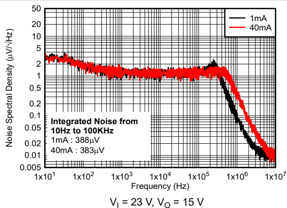
6-21. Noise Spectral Density vs Frequency and I_O for New Chip
