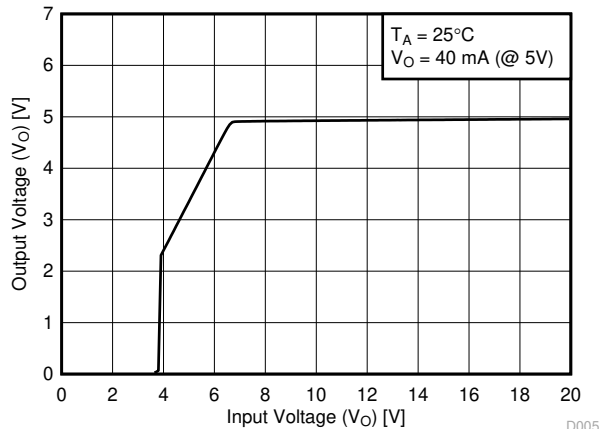
8-5. Output Voltage vs Input Voltage for New Chip
