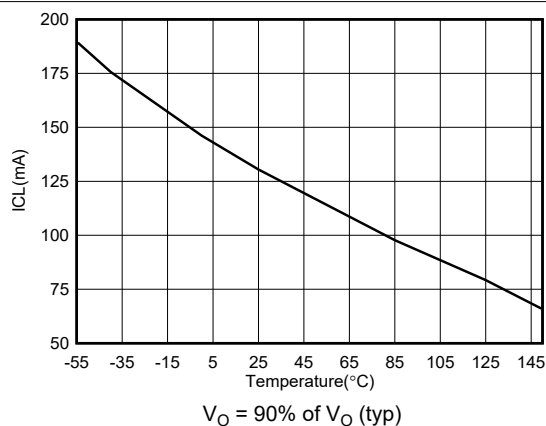
6-19. I_{CL} vs Temperature for New Chip
