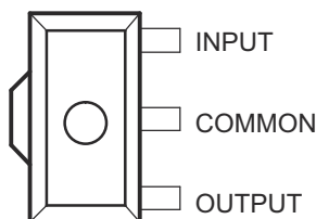
✎ 5-3. PK Package, 3-Pin SOT-89 (Top View)
