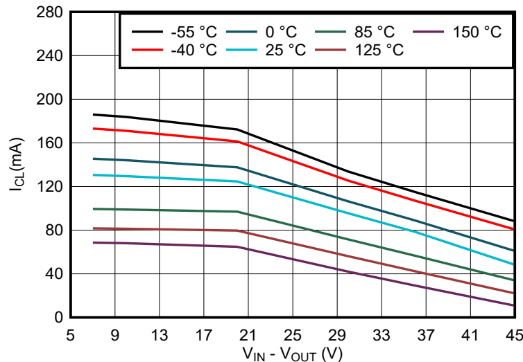
Figure 7-1. Current-Limit vs V_{Head-room} Behavior for New Chip Only
