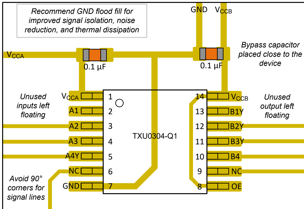
12-1. Layout Example – TXU0304-Q1
