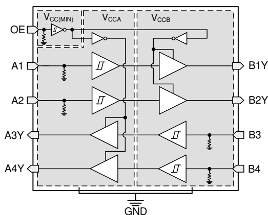
FIG 5-2. TXU0204 Functional Block Diagram
