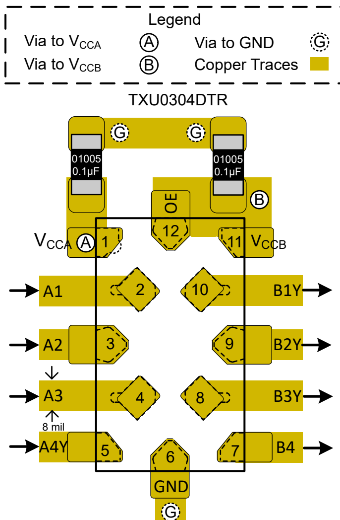
12-1. Layout Example – TXU0304
