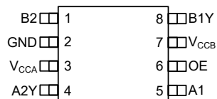
图 5-1. DCU Package, 8-Pin VSSOP (Top View)
