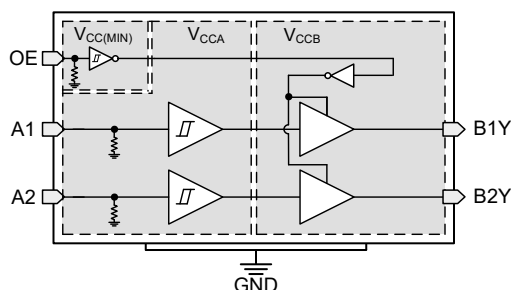
FIG 5-1. TXU0102 Functional Block Diagram
