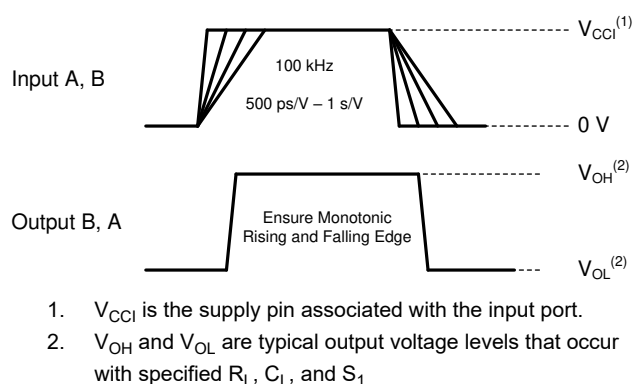
图 6-3. Input Transition Rise and Fall Rate
