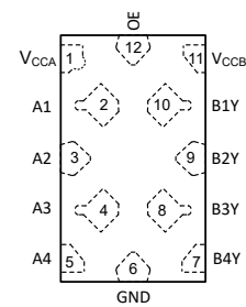
図 4-4. DTR Package 12-Pin X2SON Transparent Top View
