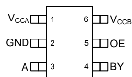
図 4-2. DCK Package, 6-Pin SC70 Transparent (Top View)
