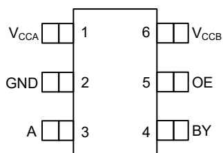
図 4-1. DBV Package, 6-Pin SOT-23 Transparent (Top View)
