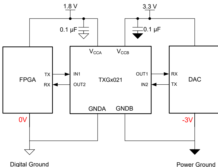
Figure 8-1. TXG1021 in Test and Measurement
