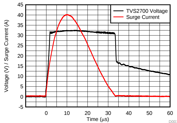
FIG 11. TVS2700 Surge Response at 40 A
