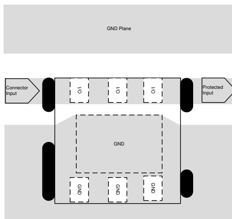
9-3. TVS2200 Layout
