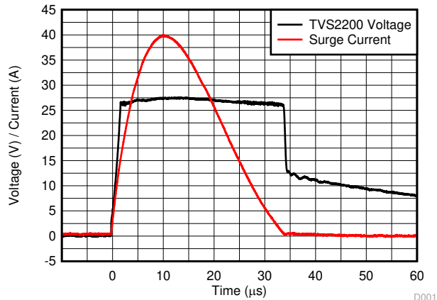
9-2. TVS2200 Surge Response at 40 A
