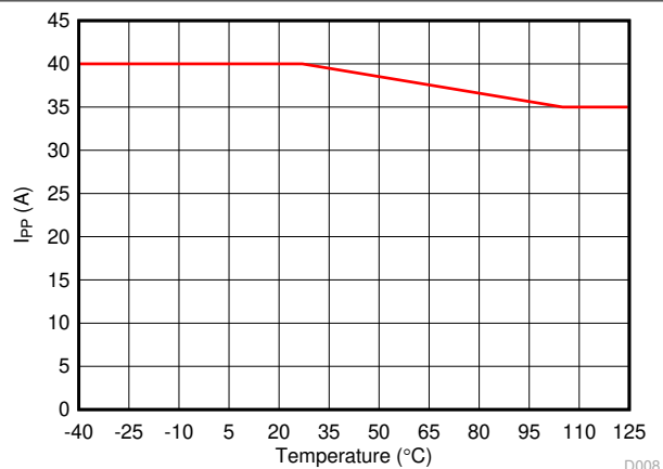
7-8. Maximum Surge Current (8/20 \mu s) vs Temperature
