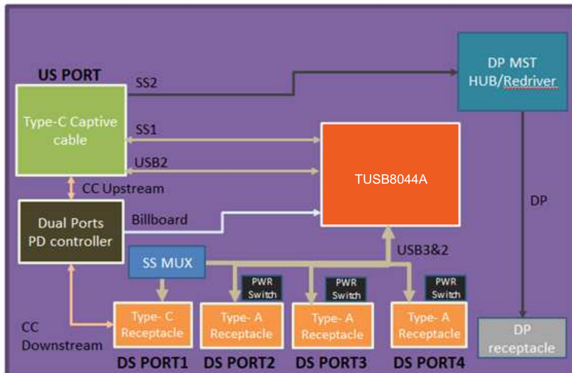
☒ 36. Discrete USB Hub Product
