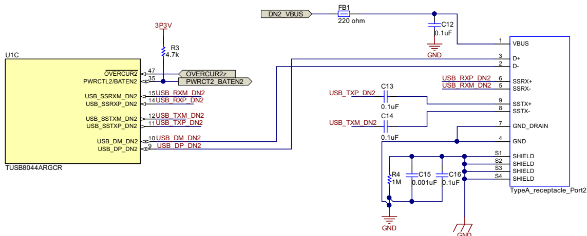
FIG 39. Downstream Port 2 Implementation
