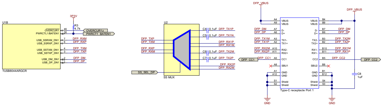
FIG 38. Downstream Port 1 Implementation
