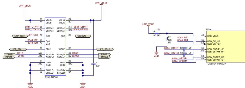
☒ 37. Upstream Port Implementation
