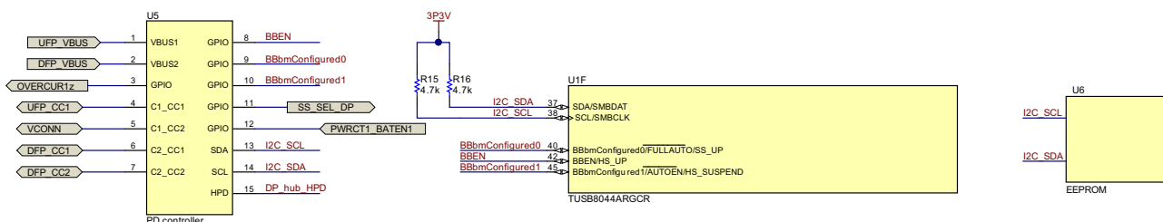
43. PD Controller and EEPROM Implementation
