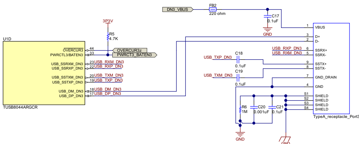
FIG 40. Downstream Port 3 Implementation
