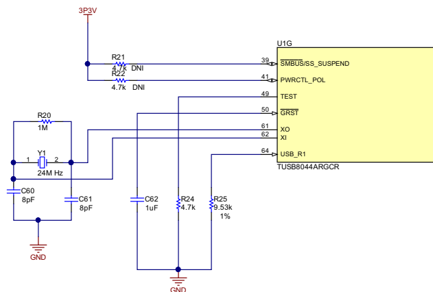
FIG 46. Clock, Reset, and Misc
