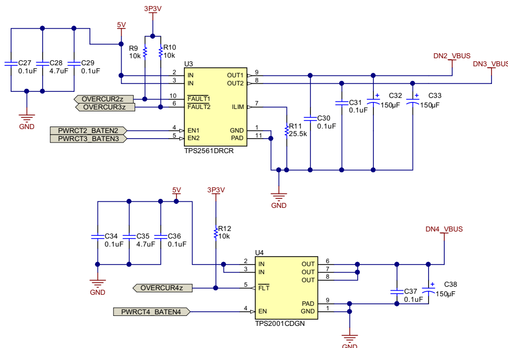
❏ 42. VBUS Power Switch Implementation
