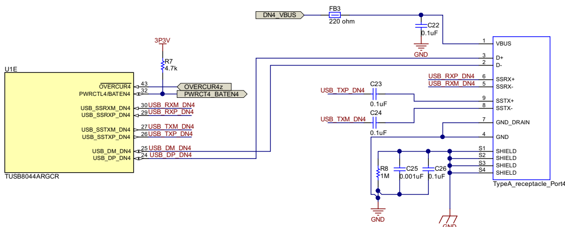
FIG 41. Downstream Port 4 Implementation
