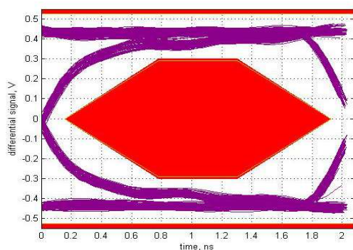
図 54. High-Speed Downstream Port 1
