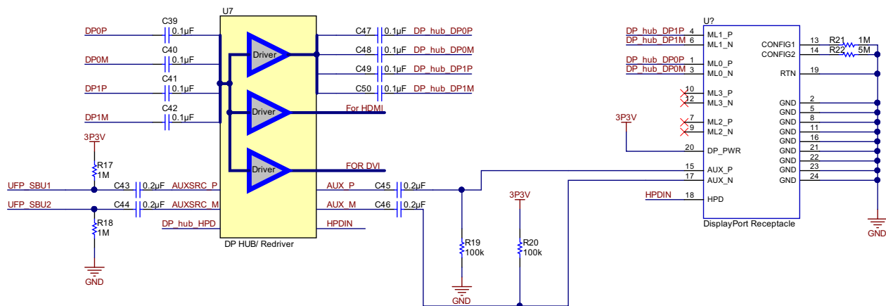
FIG 45. DisplayPort Implementation
