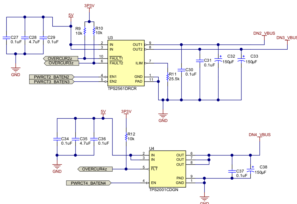
Figure 41. VBUS Power Switch Implementation
