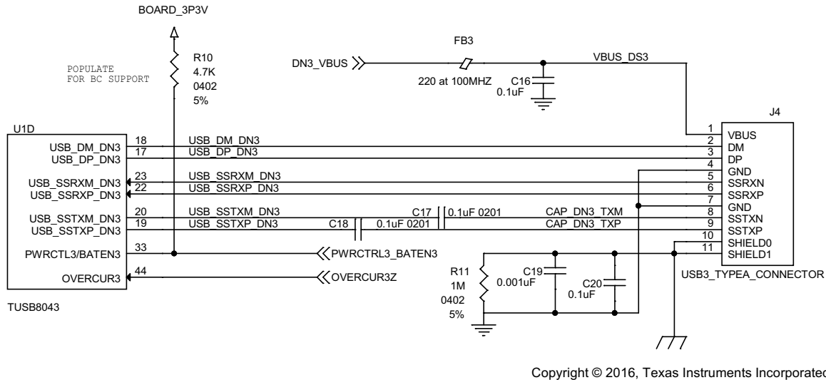
Figure 31. Downstream Port 3 Implementation
