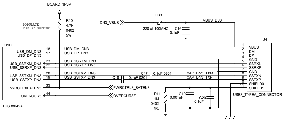
9-5. Downstream Port 3 Implementation
