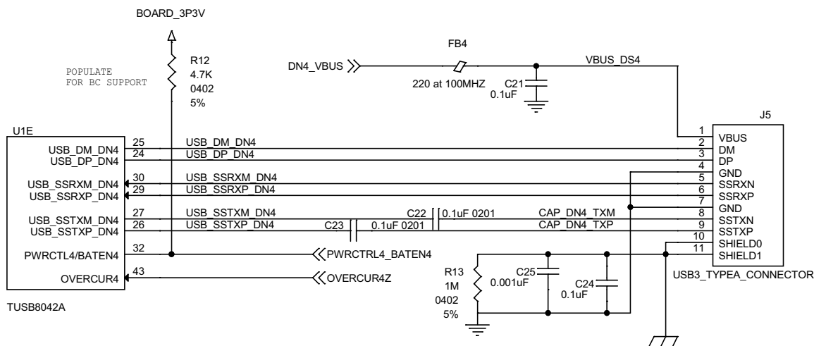
9-6. Downstream Port 4 Implementation
