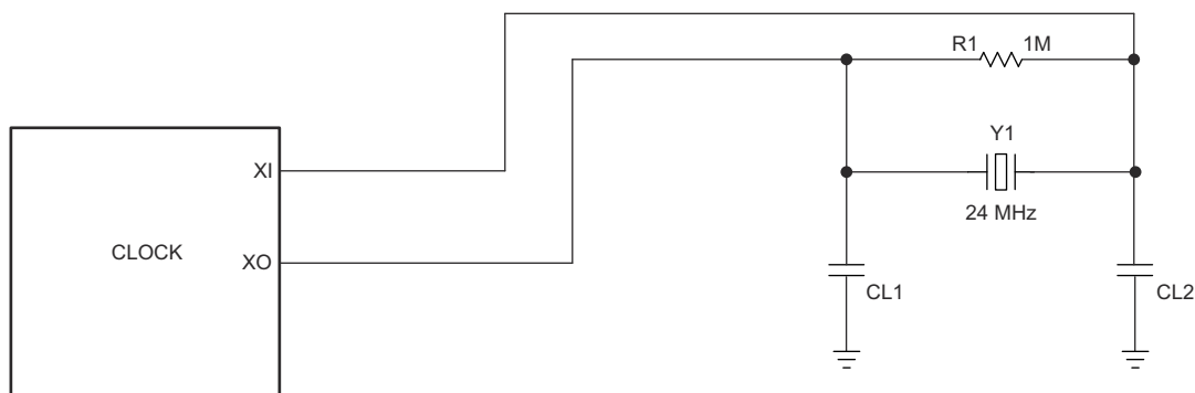
7-1. TUSB8042A Clock
