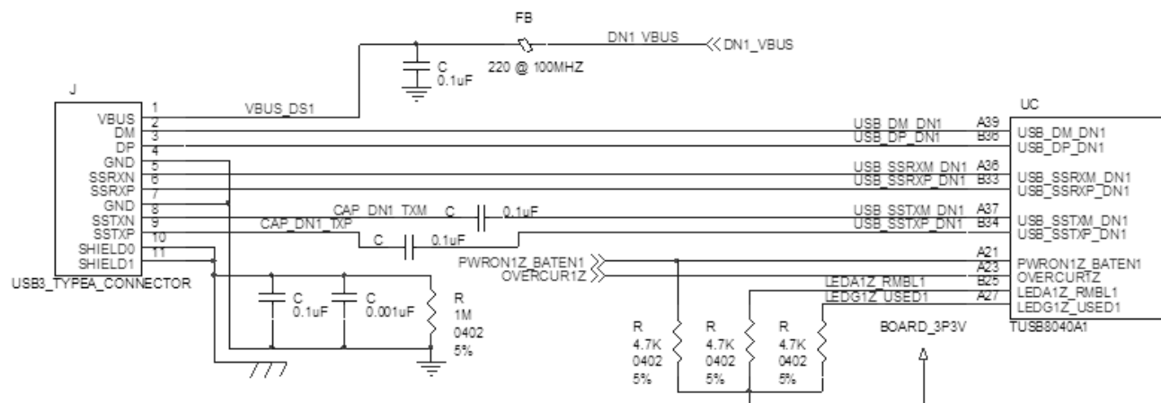
FIG 8-5. Downstream Port 3 Implementation
