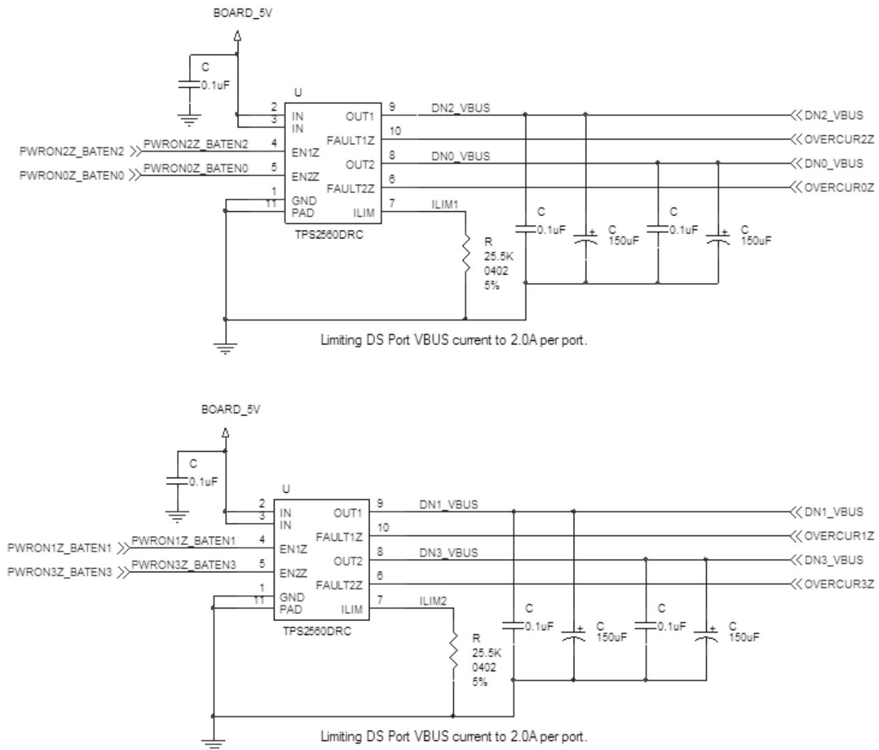
8-7. VBUS Power Switch Implementation
