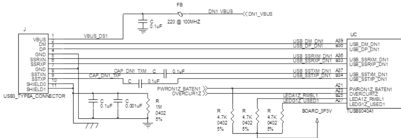
FIG 8-4. Downstream Port 2 Implementation
