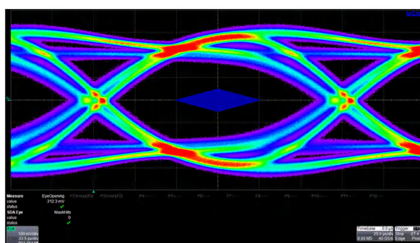
8-13. Downstream Port 3
