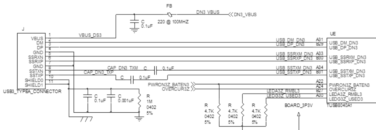
FIG 8-6. Downstream Port 4 Implementation
