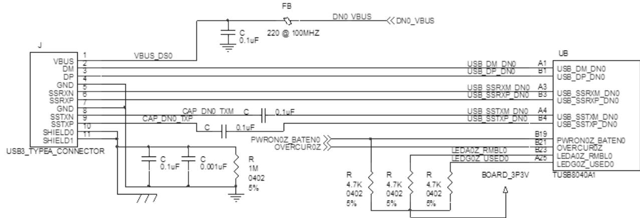
FIG 8-3. Downstream Port 1 Implementation
