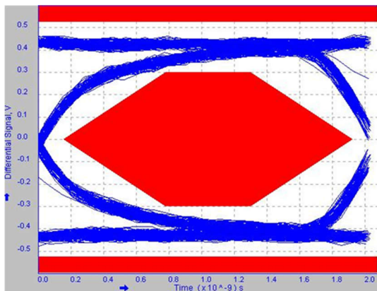
図 7-12. High-Speed Downstream Port 1
