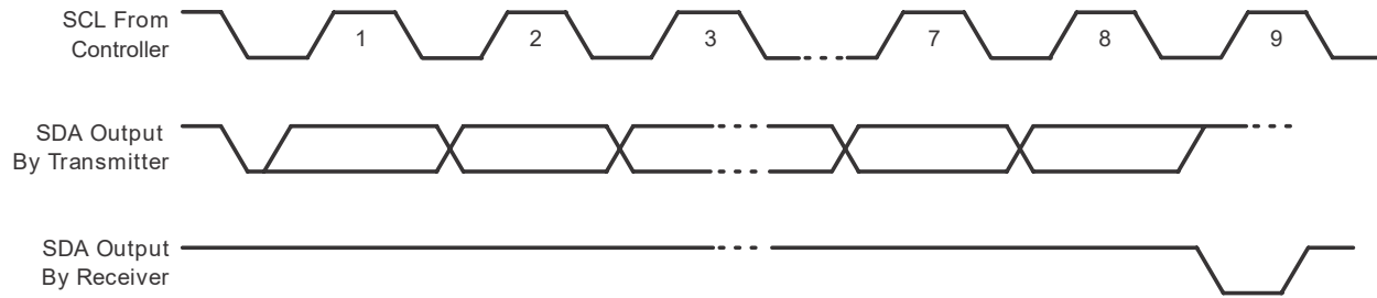
FIG 6-4. Serial-Bus Protocol Acknowledge
