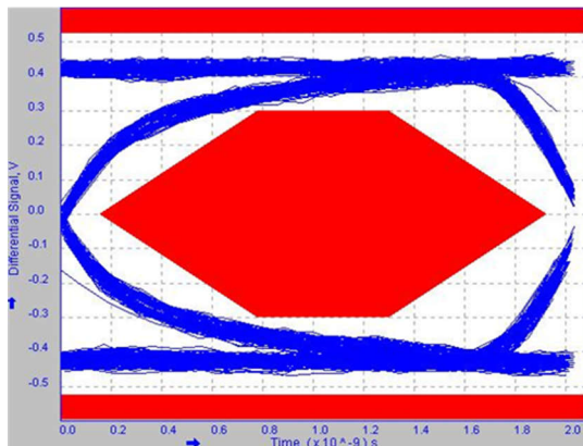
図 7-14. High-Speed Downstream Port 3
