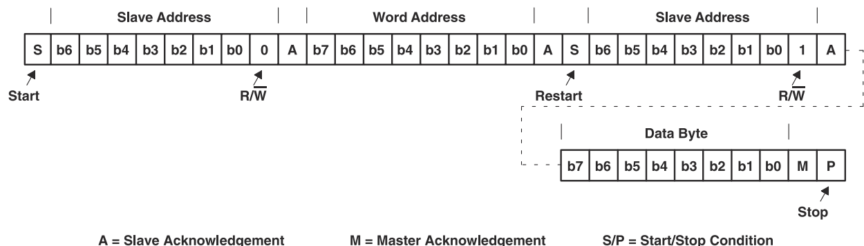
FIG 6-6. Serial-Bus Protocol – Byte Read
