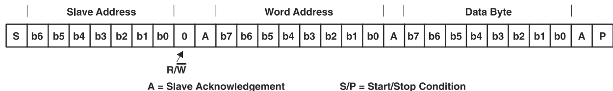
FIG 6-5. Serial-Bus Protocol – Byte Write
