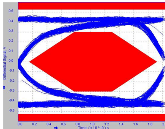
図 7-13. High-Speed Downstream Port 2
