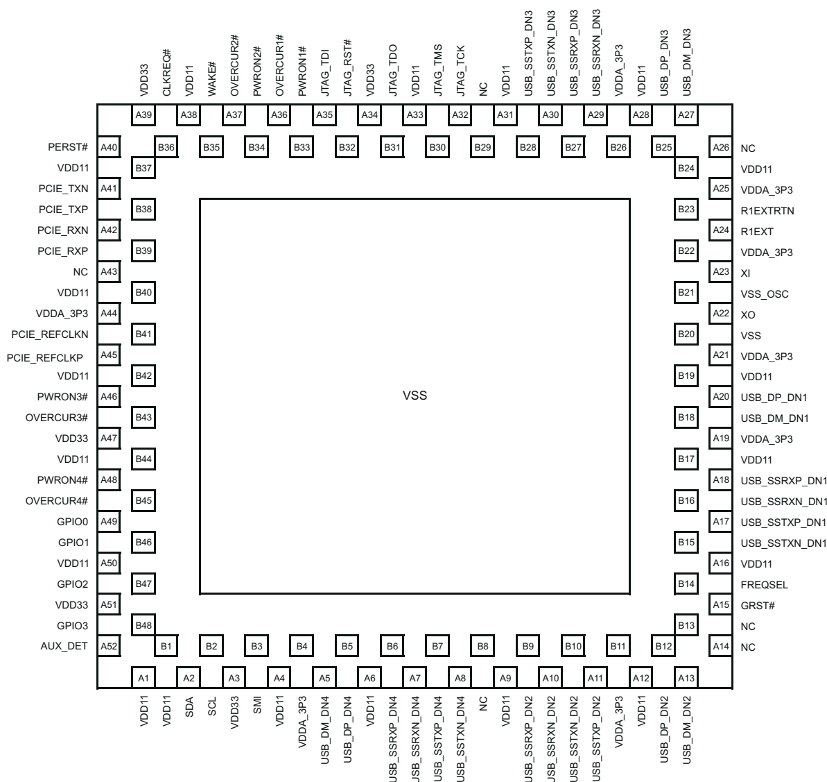
図 4-2. RKM Package, 100-Pin WQFN-MR Exposed Thermal Pad TUSB7340 (Top View)
