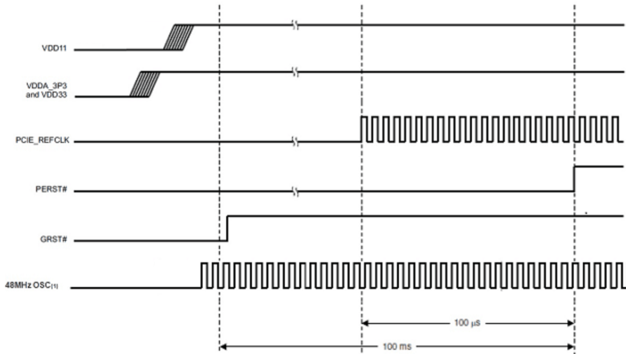
図 7-16. Power-Up Sequence
