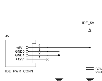
OPTION 2: 5V FROM IDE CONNECTOR
