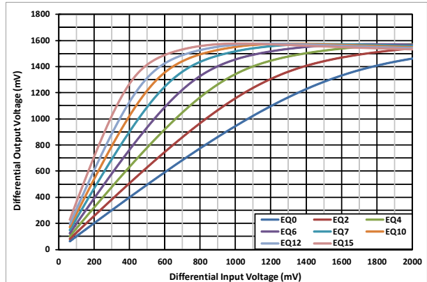
Figure 6-6. USB RX (UFP) Linearity Curves at 2.5 GHz
