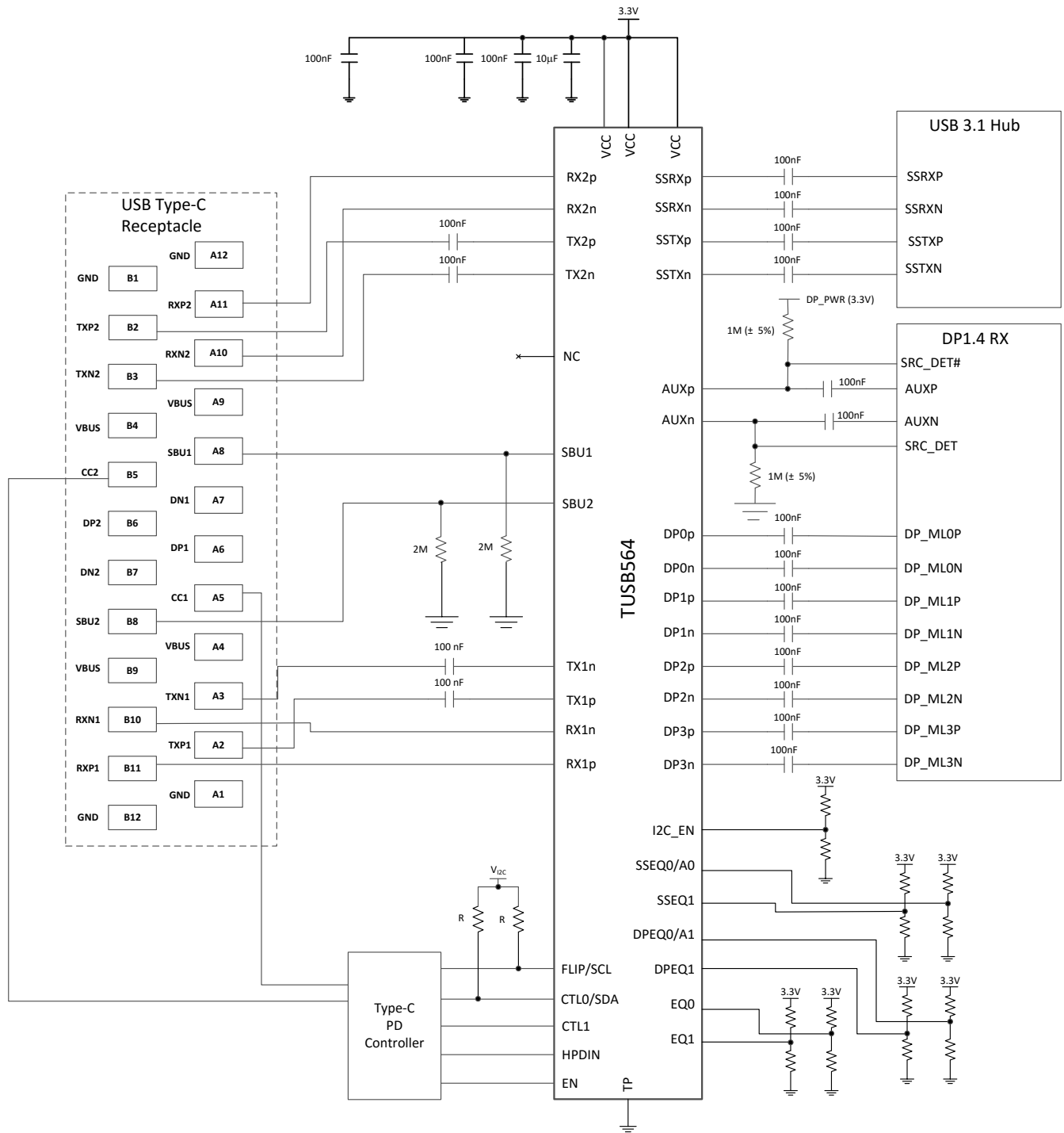
9-2. Application Circuit
