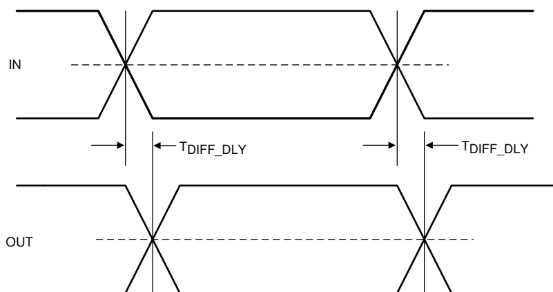
Figure 7-3. Propagation Delay
