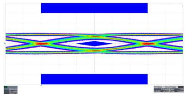
Figure 7. After Re-Driver EQ(6dB), Input = 20", Output = 4"+3m Cable
