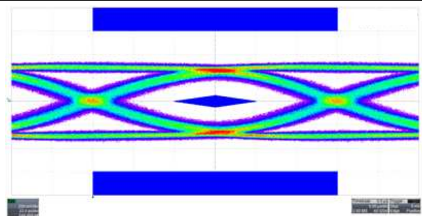
Figure 5. After Re-Driver EQ(3dB), Input = 12", Output = 4"+3m Cable
