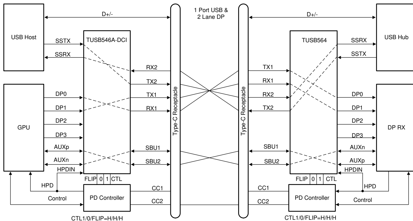
Figure 33. USB 3.1 + 2 Lane DP – Flip (CTL1 = H, CTL0 = H, FLIP = H)
