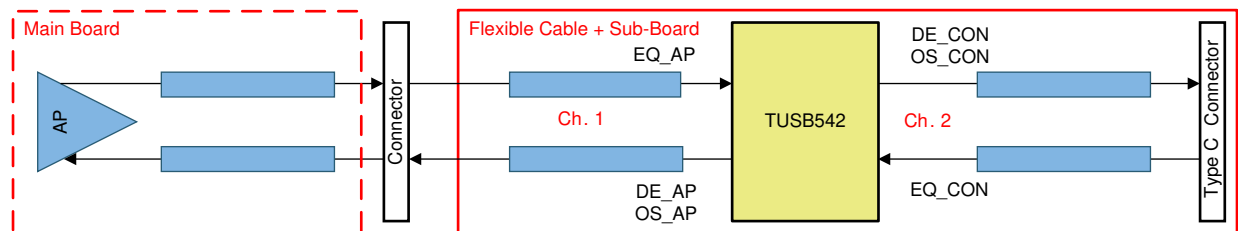
図 6-1. Typical Channels
