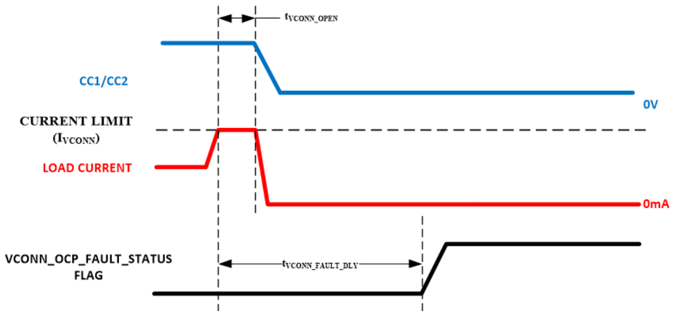
図 2. VCONN Fault Timing
