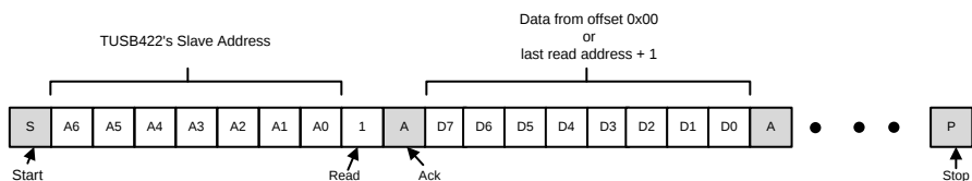
✎ 7. I2C Read Without Repeated Start
