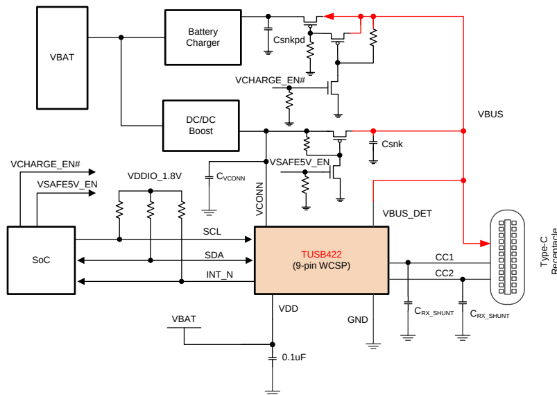
図 76. TUSB422 in DRP Application
