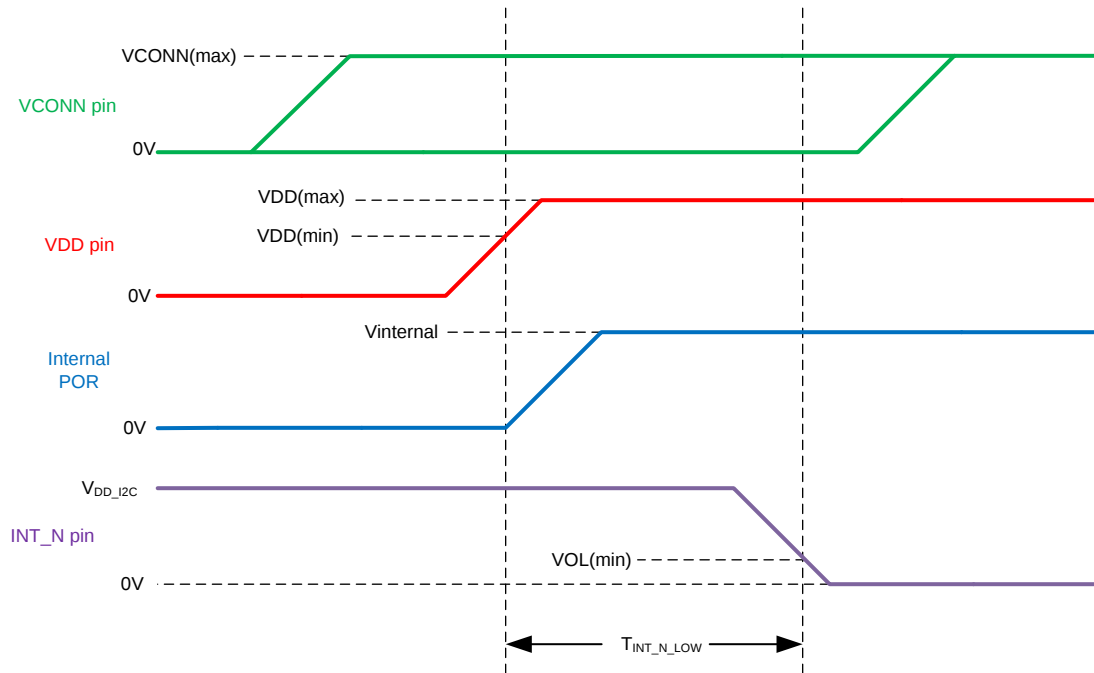
図 1. Power-Up Timing
