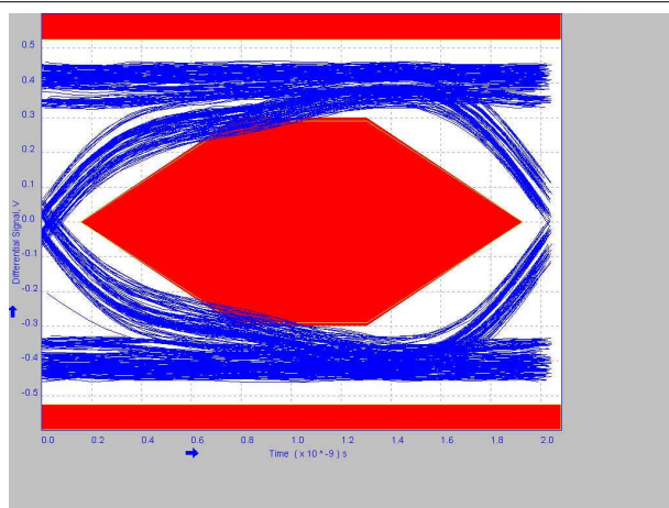
9-20. 4 Meter Post-Channel Without TUSB217A
