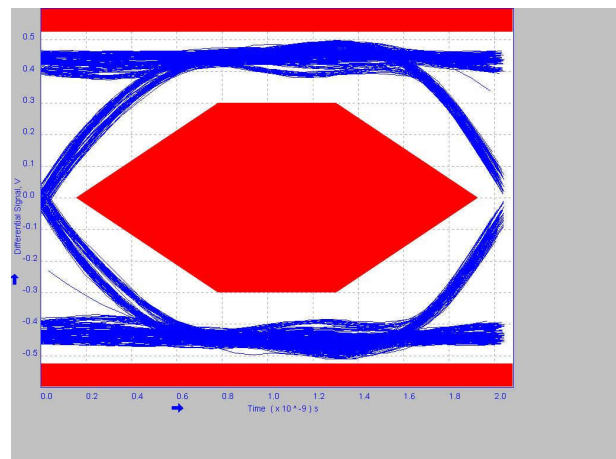
9-13. 6 Inches Post-Channel With TUSB217A BOOST=0 RX_SEN=HIGH
