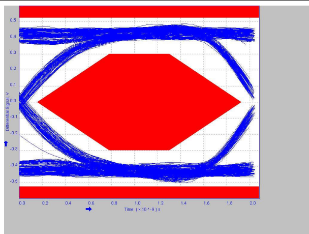
9-16. 1 Meter Post-Channel With TUSB217A BOOST=0 RX_SEN=HIGH
