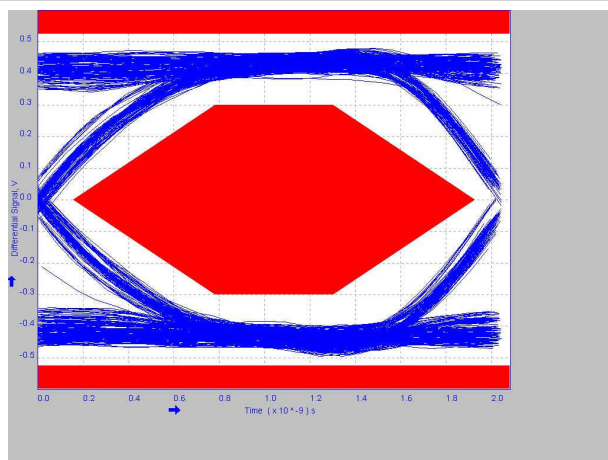
9-18. 2 Meter Post-Channel With TUSB217A BOOST=1 RX_SEN=MED
