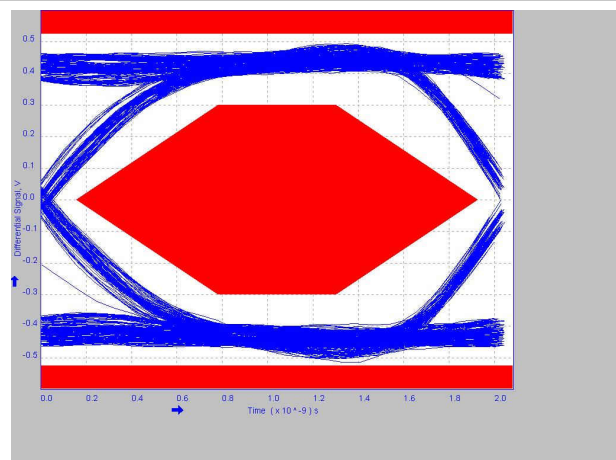
9-15. 1 Meter Post-Channel With TUSB217A BOOST=0 RX_SEN=MED
