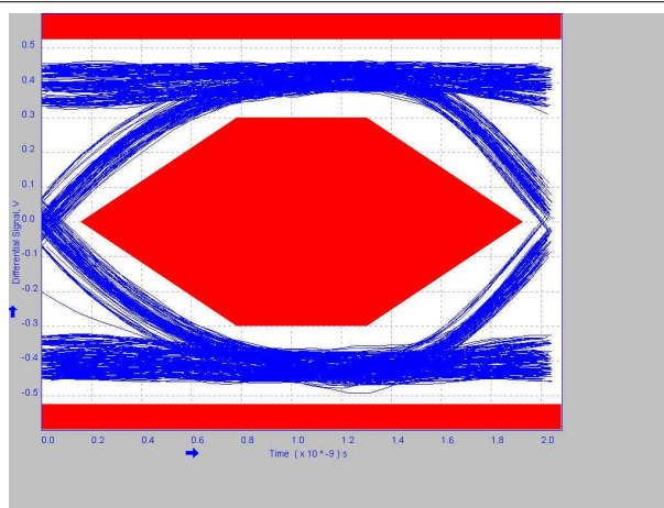
9-21. 4 Meter Post-Channel With TUSB217A BOOST=2 RX_SEN=MED
