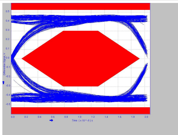
9-14. 1 Meter Post-Channel Without TUSB217A
