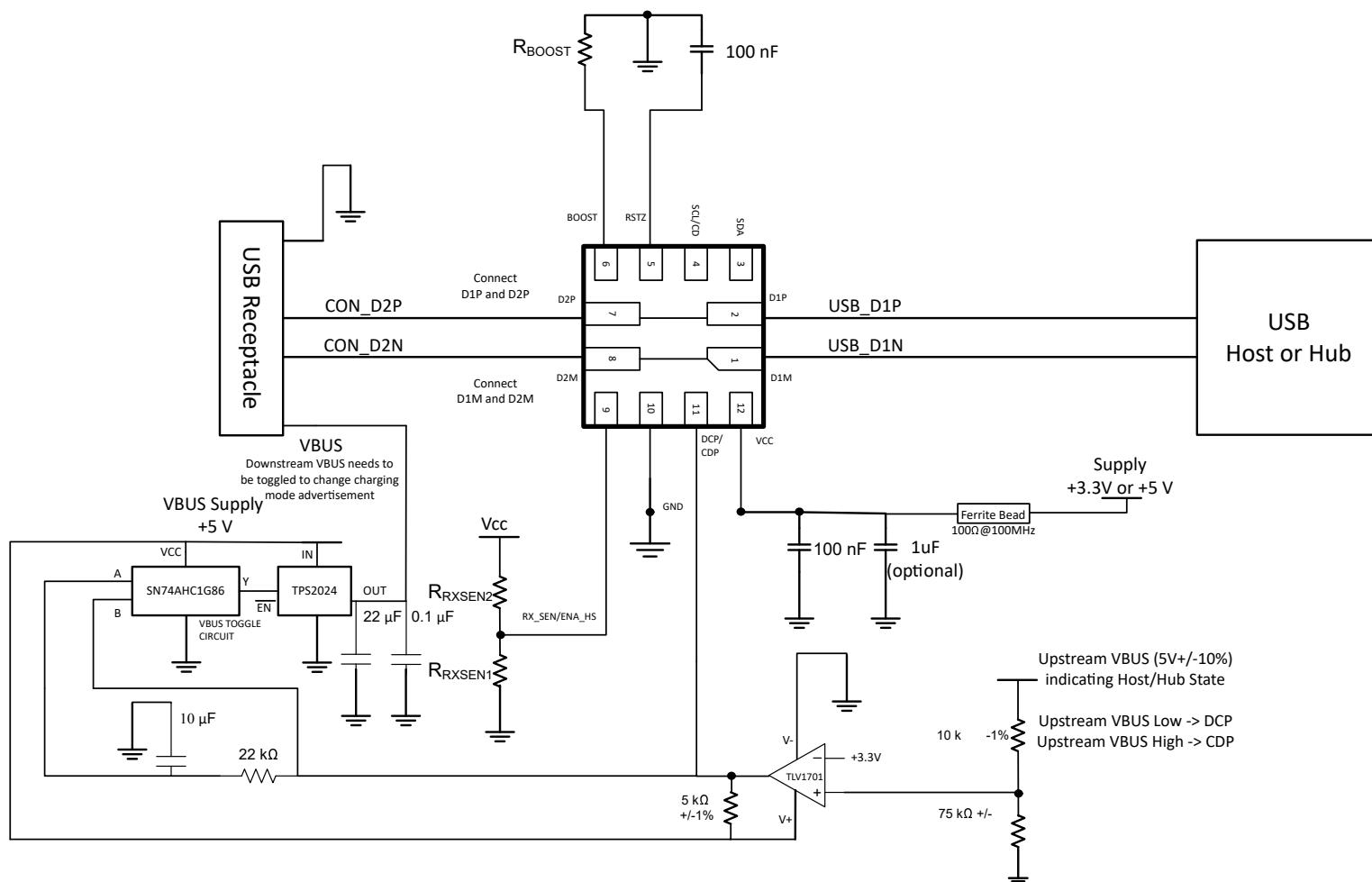
9-1. TUSB217A: A Reference Schematic (Design Example with DCP/CDP Dynamic Switching). Downstream VBUS Needs to be Toggled if Upstream VBUS State Changes for BC 1.2 Controller to Change DCP/CDP Advertisement.
