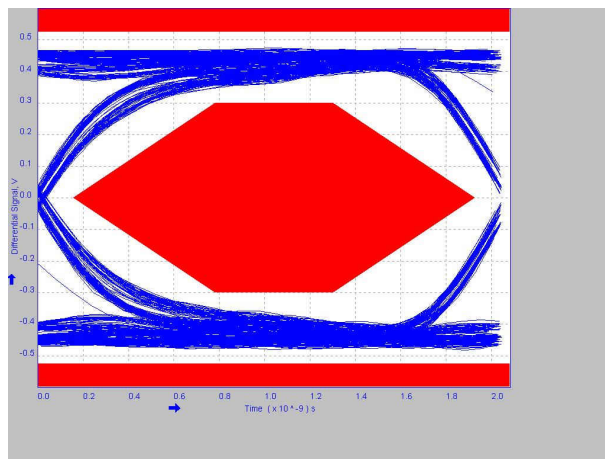
9-12. 6 Inches Post Channel Without TUSB217A
