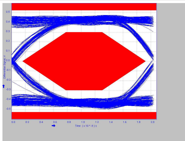
9-19. 2 Meter Post-Channel With TUSB217A BOOST=1 RX_SEN=HIGH
