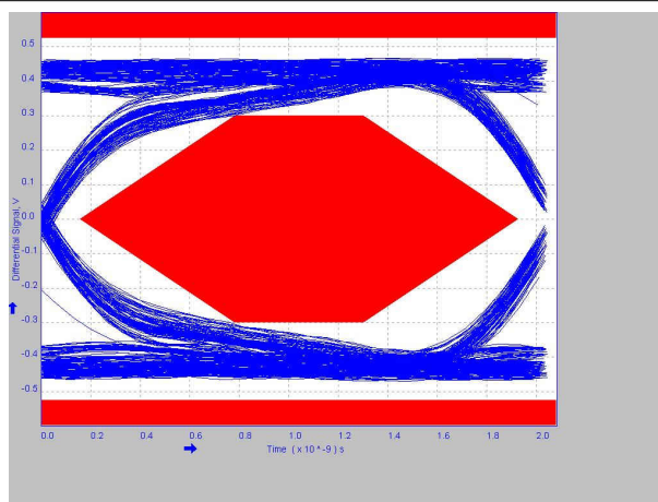
9-17. 2 Meter Post-Channel Without TUSB217A
