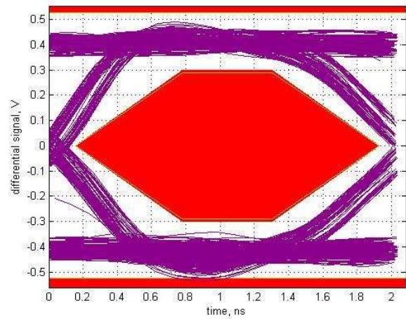
FIG 19. Low DC Boost, AC Boost Level 3
