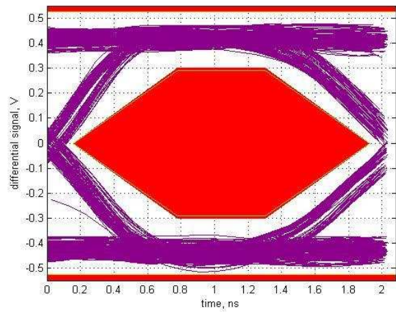
FIG 17. Mid DC Boost, AC Boost Level 2
