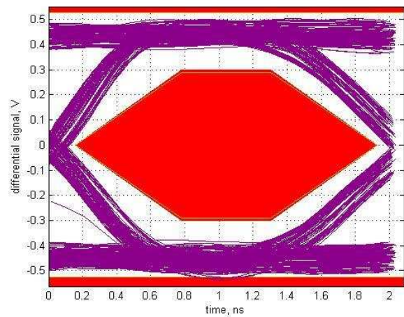
FIG 21. High DC Boost, AC Boost Level 3
