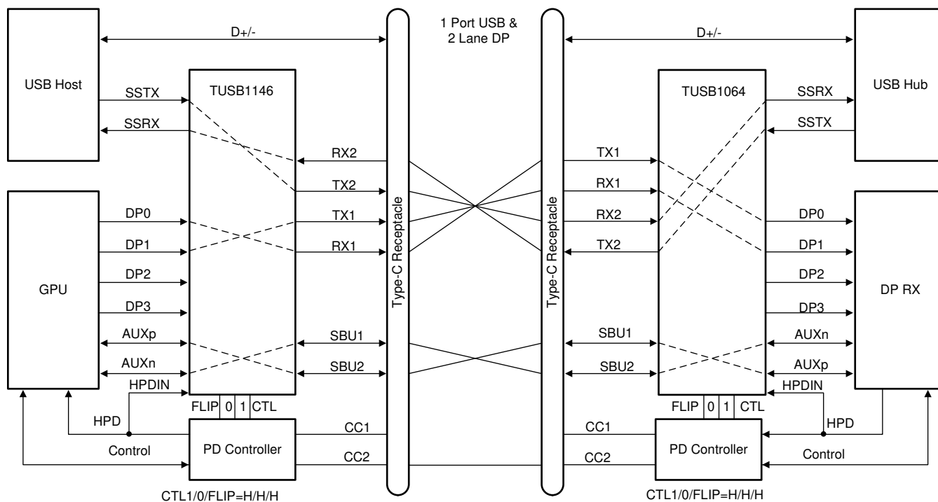
Figure 39. USB 3.1 + 2 Lane DP – Flip (CTL1 = H, CTL0 = H, FLIP = H)
