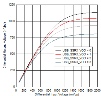
Figure 14. USB SSRX VOD Linearity Settings at 5GHz
