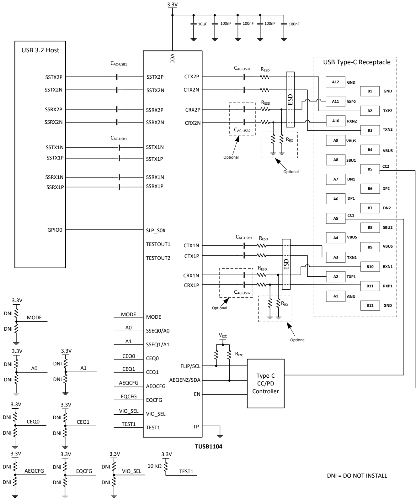
図 8-2. Application Circuit
