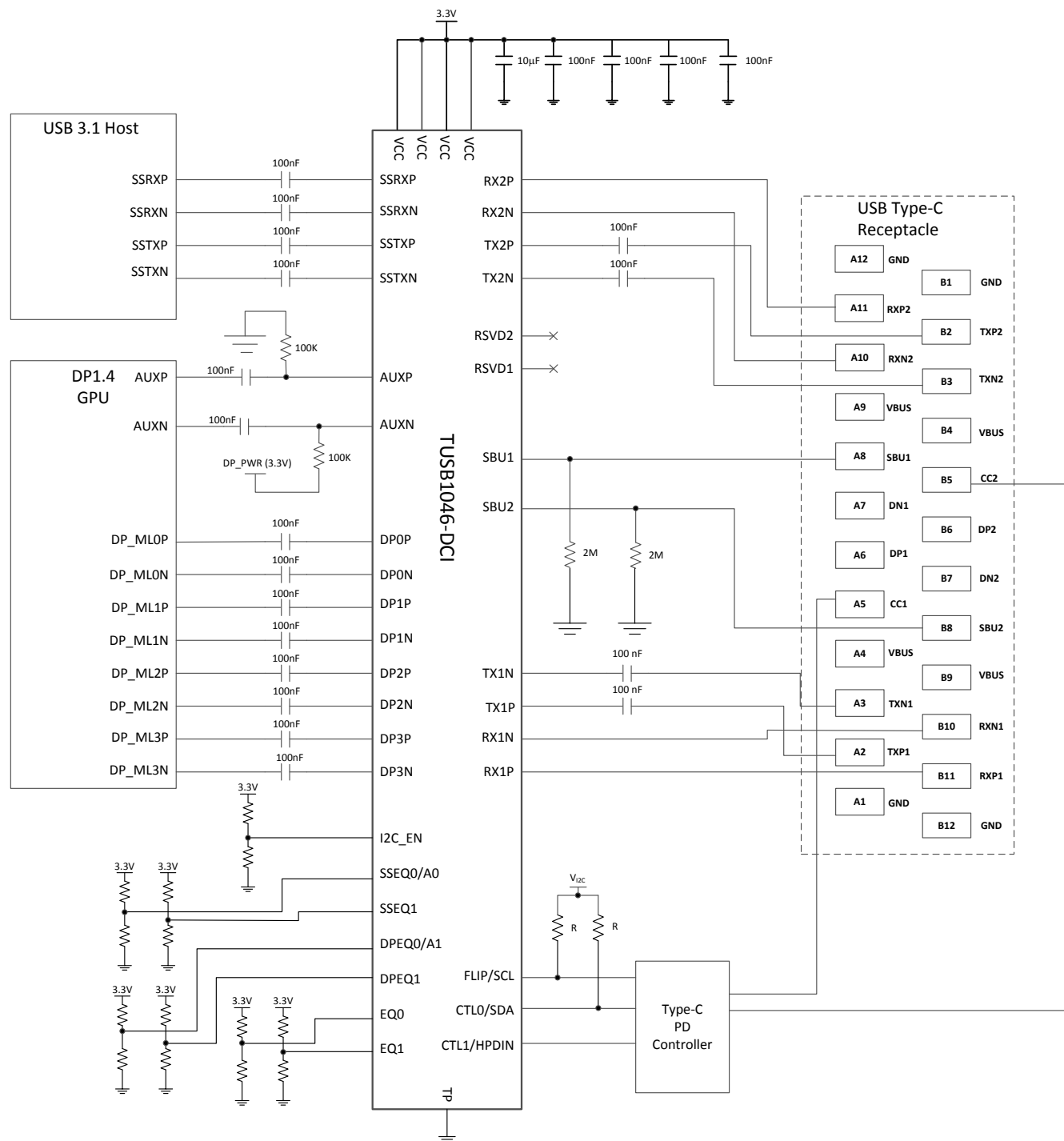
8-2. Application Circuit
