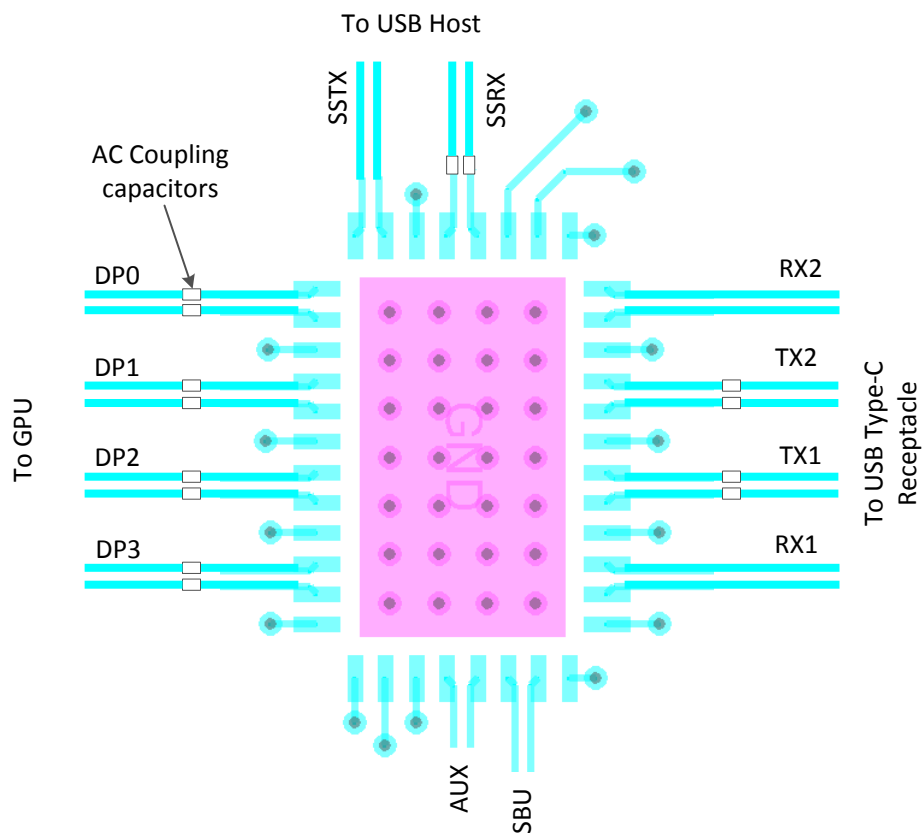
10-1. Layout Example
