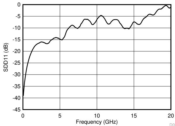
図 5-11. Input Return Loss Performance of the Upstream Ports
