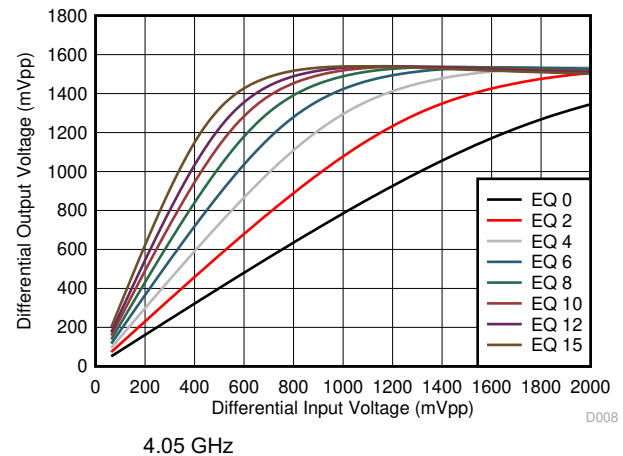
図 5-14. Downstream-to-Upstream Linearity Performance at 4.05 GHz
