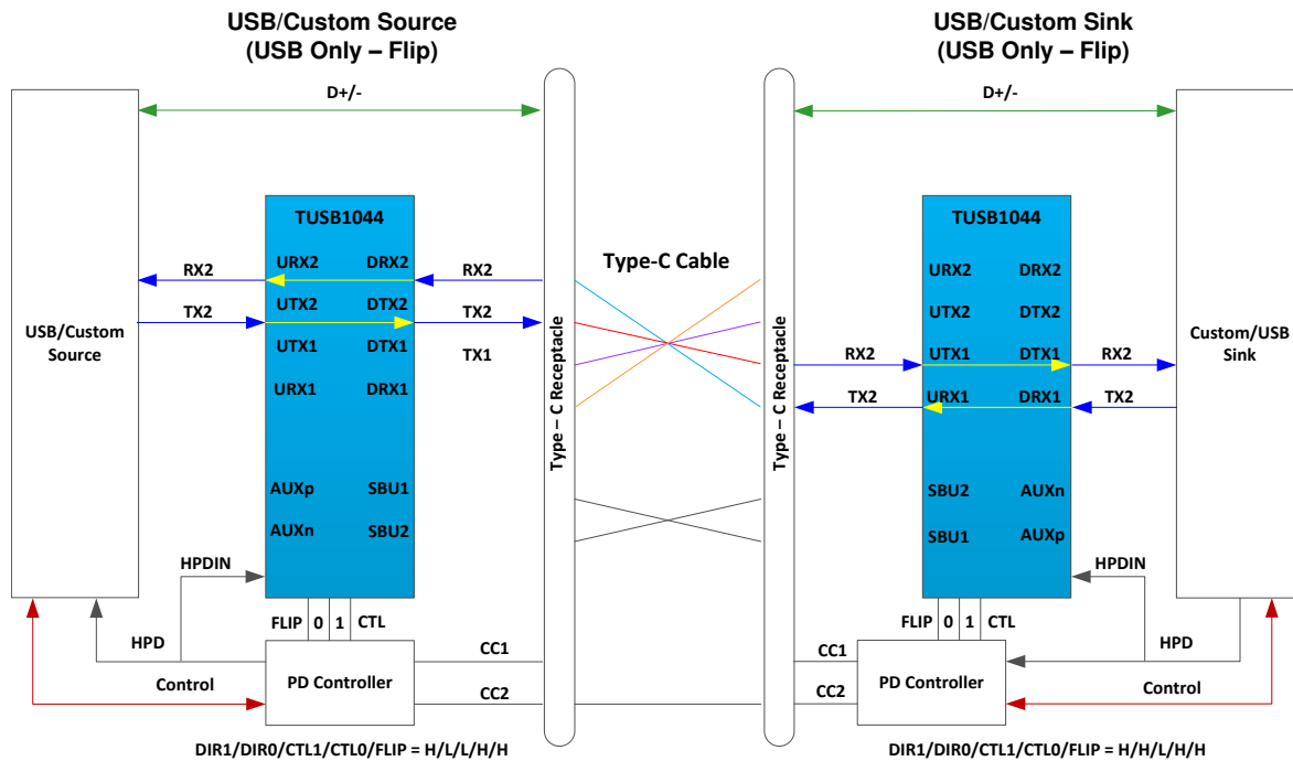
図 7-11. USB3.1 Only – With Flip
