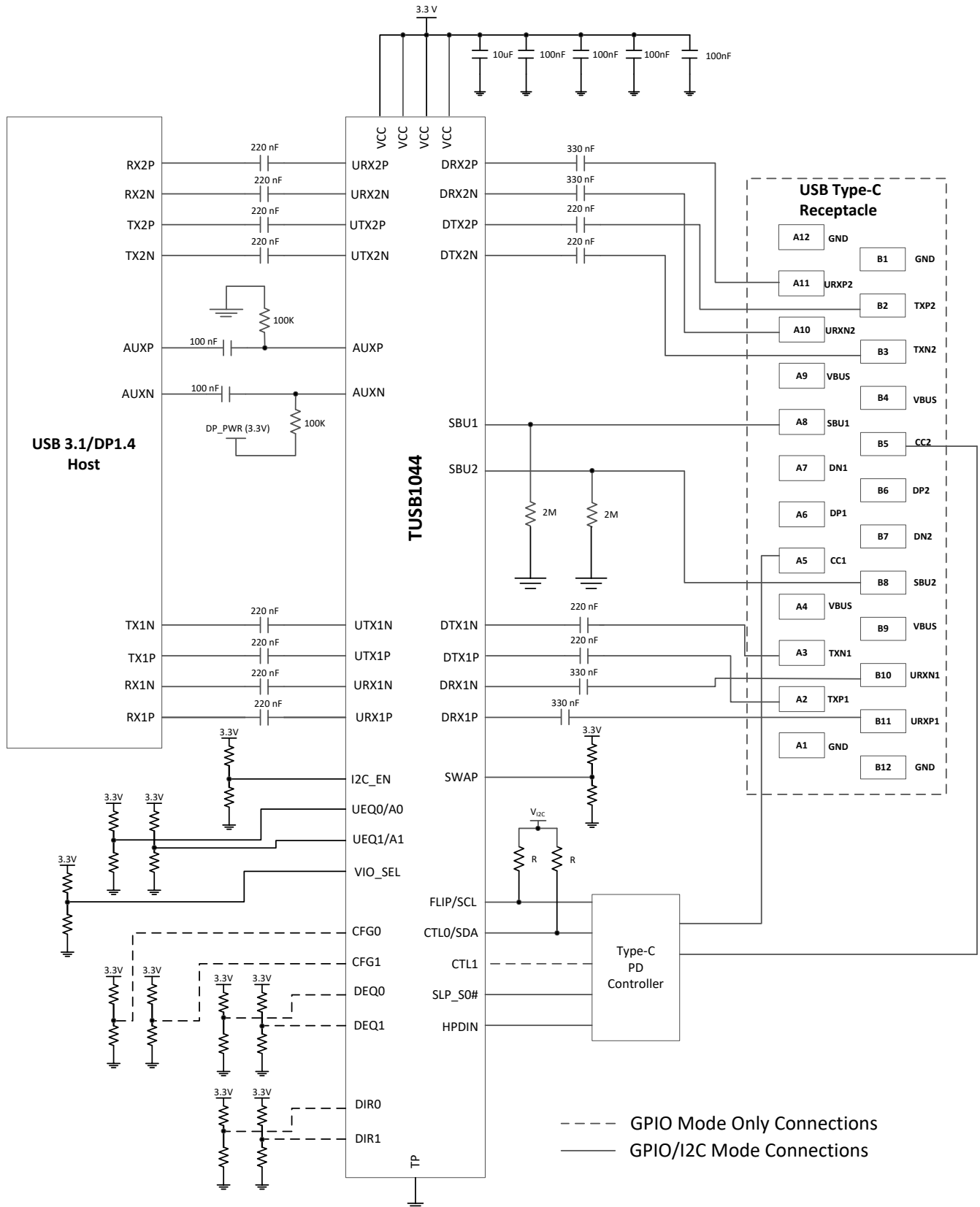
図 7-2. Typical Application Circuit
