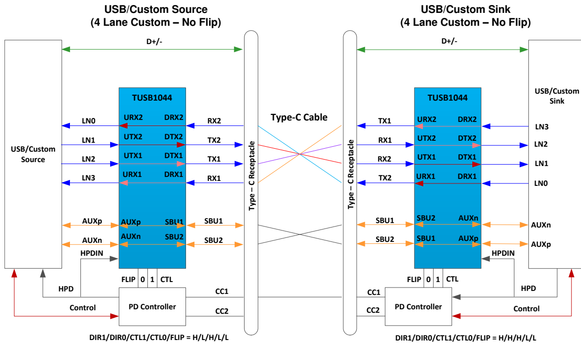
図 7-16. Four Lane Custom Alternate Mode – No Flip
