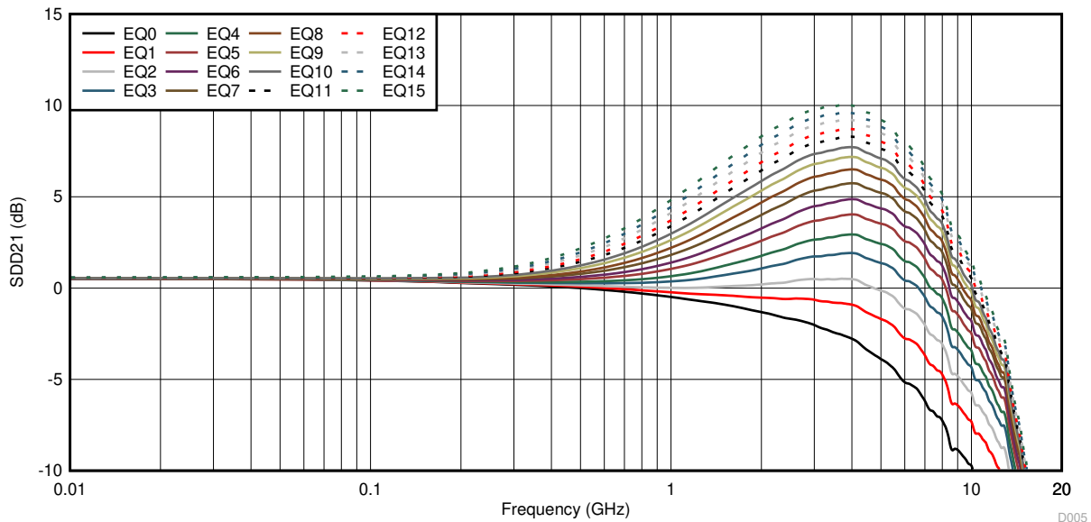
図 5-21. Upstream-to-Downstream EQ Settings Curves
