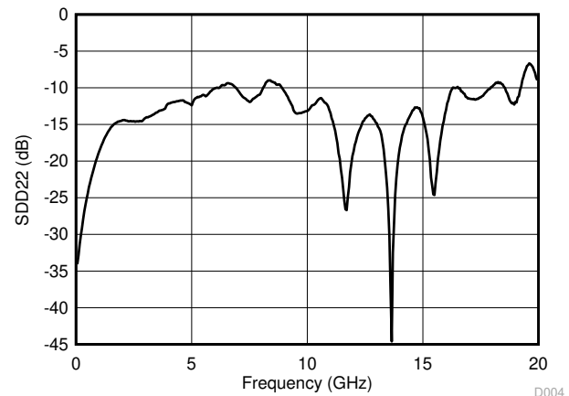
図 5-12. Output Return Loss Performance of the Upstream Ports
