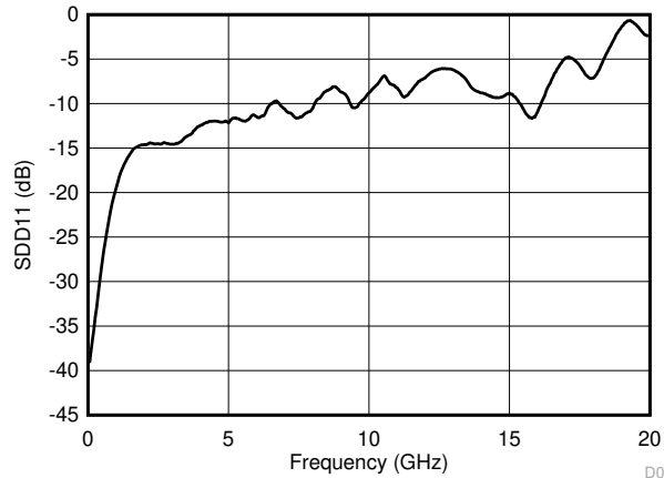
図 5-9. Input Return Loss Performance of the Downstream Ports
