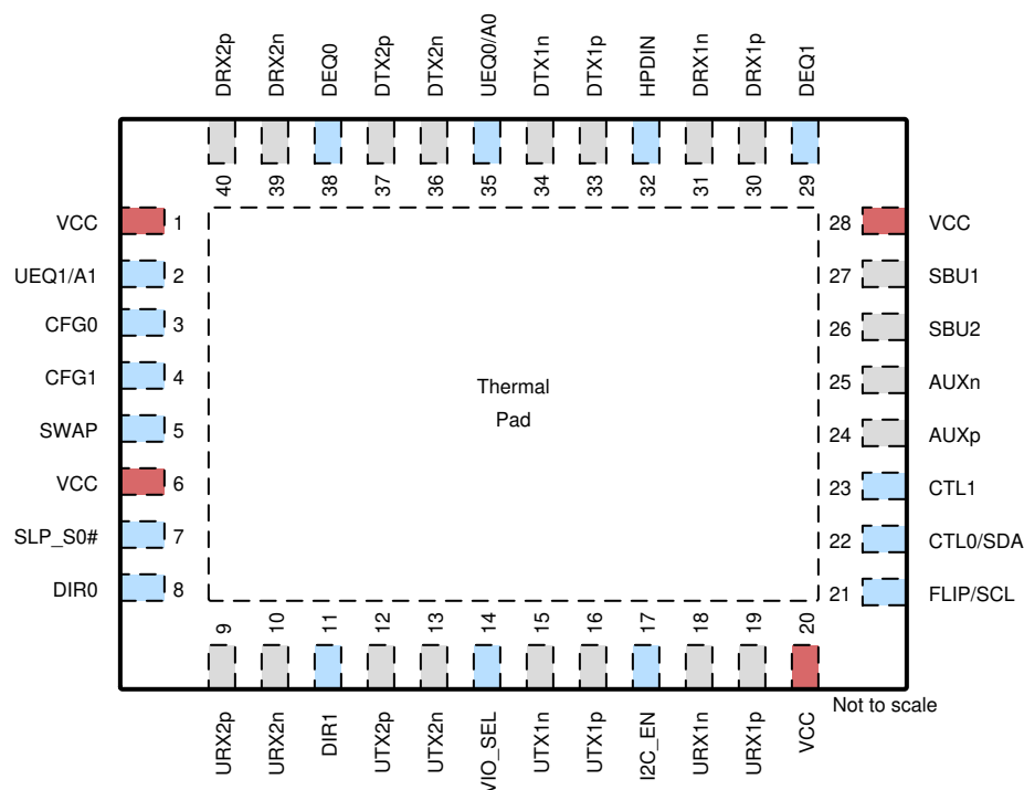
図 4-1. RNQ Package 40-Pin (WQFN) Top View
