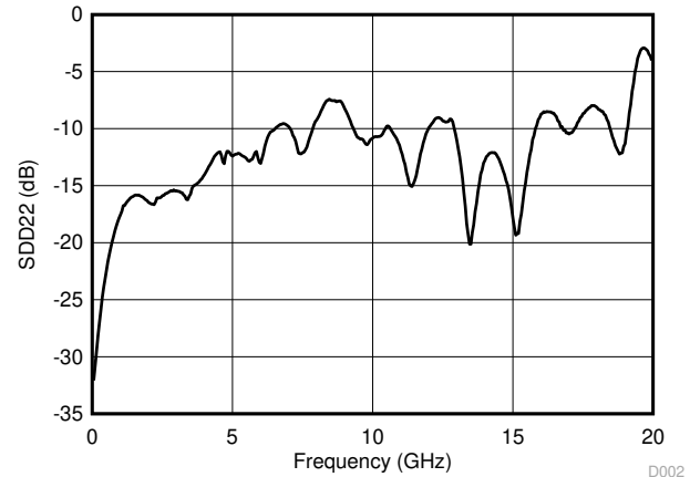
図 5-10. Output Return Loss Performance of the Downstream Ports
