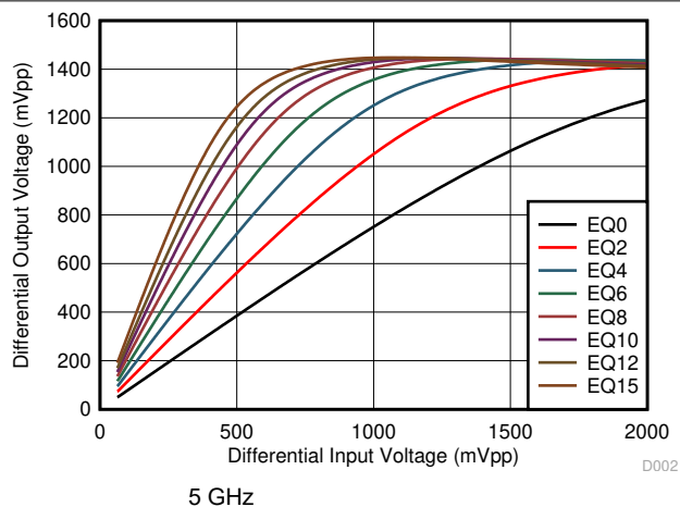
5-16. Upstream-to-Downstream Linearity Performance at 5 GHz
