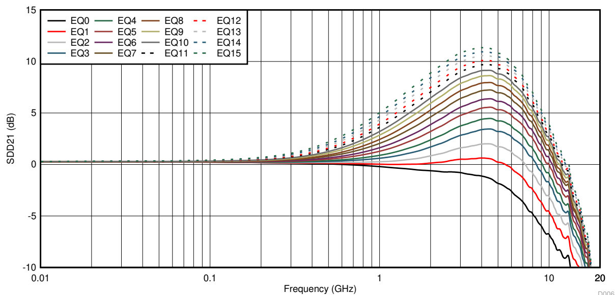
図 5-22. Downstream-to-Upstream EQ Settings Curves
