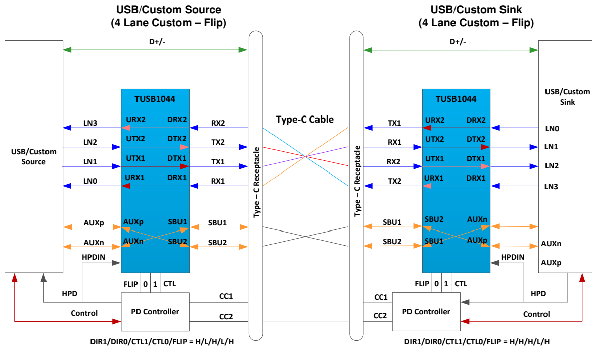
図 7-17. Four Lane Custom Alternate Mode – With Flip
