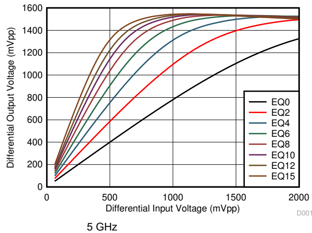
図 5-13. Downstream-to-Upstream Linearity Performance at 5 GHz
