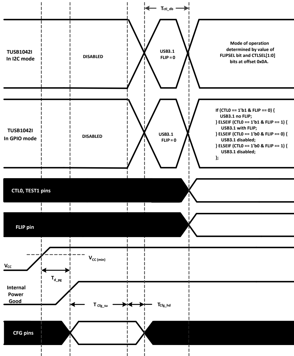
图 14. Power-Up Timing
